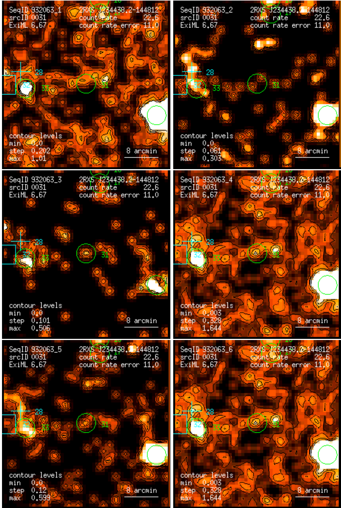
Figure 31: RASS 932063: detection 0031: band rate images, Gaussian filter: (1) PSPC channels 11 – 41, (2) 52 – 90, (3) 91 – 201, (4) 11 – 235, (5) 52 – 201, (6) 11 – 201. Broad band rates in counts/ks. Band rate contour levels in counts/ks/arcmin 2 .
