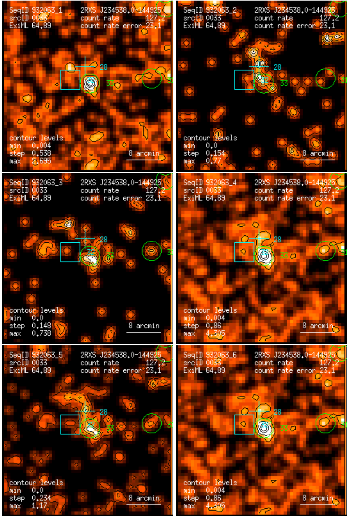
Figure 33: RASS 932063: detection 0033: band rate images, Gaussian filter: (1) PSPC channels 11 – 41, (2) 52 – 90, (3) 91 – 201, (4) 11 – 235, (5) 52 – 201, (6) 11 – 201. Broad band rates in counts/ks. Band rate contour levels in counts/ks/arcmin 2 .
