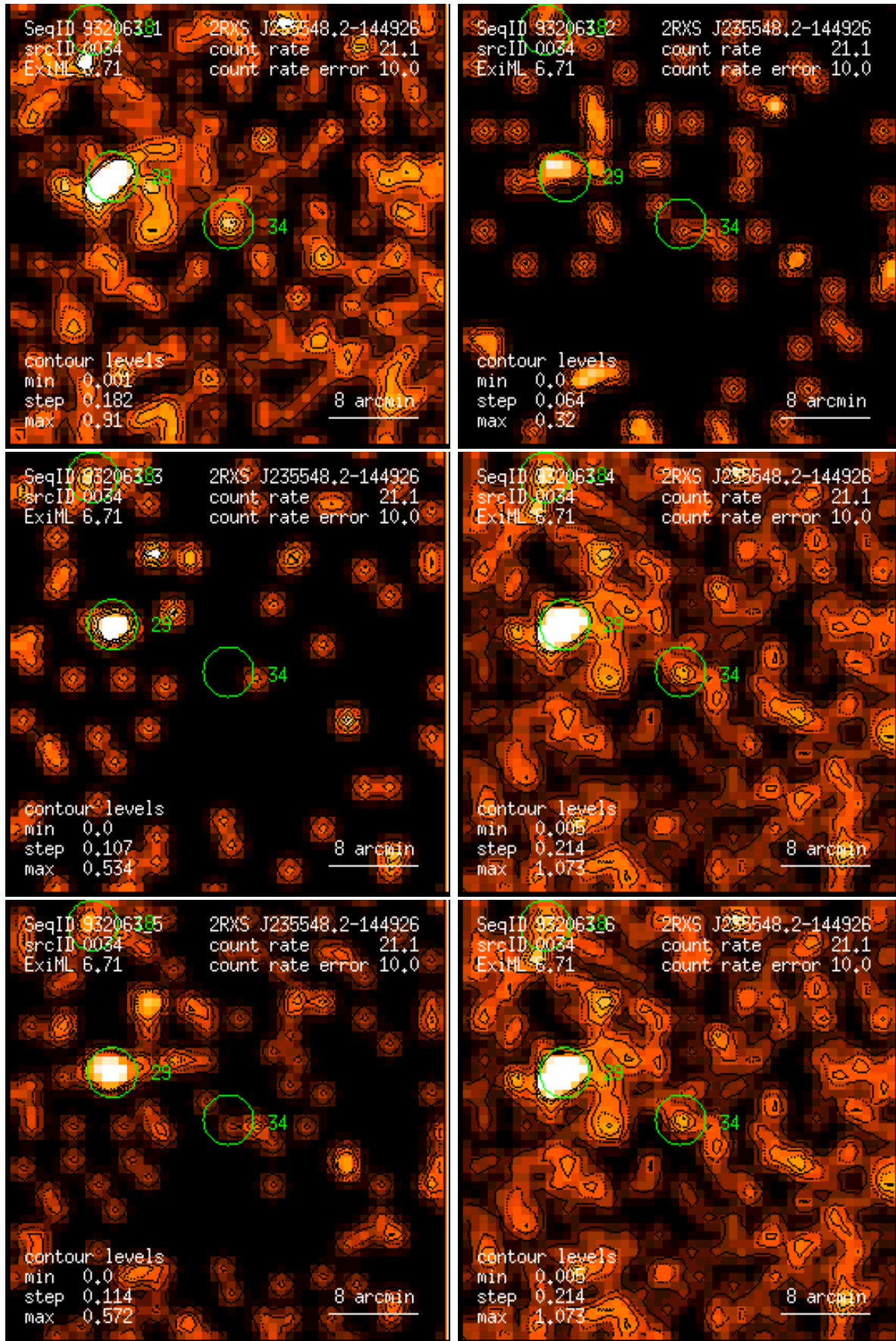
Figure 34: RASS 932063: detection 0034: band rate images, Gaussian filter: (1) PSPC channels 11 – 41, (2) 52 – 90, (3) 91 – 201, (4) 11 – 235, (5) 52 – 201, (6) 11 – 201. Broad band rates in counts/ks. Band rate contour levels in counts/ks/arcmin 2 .
