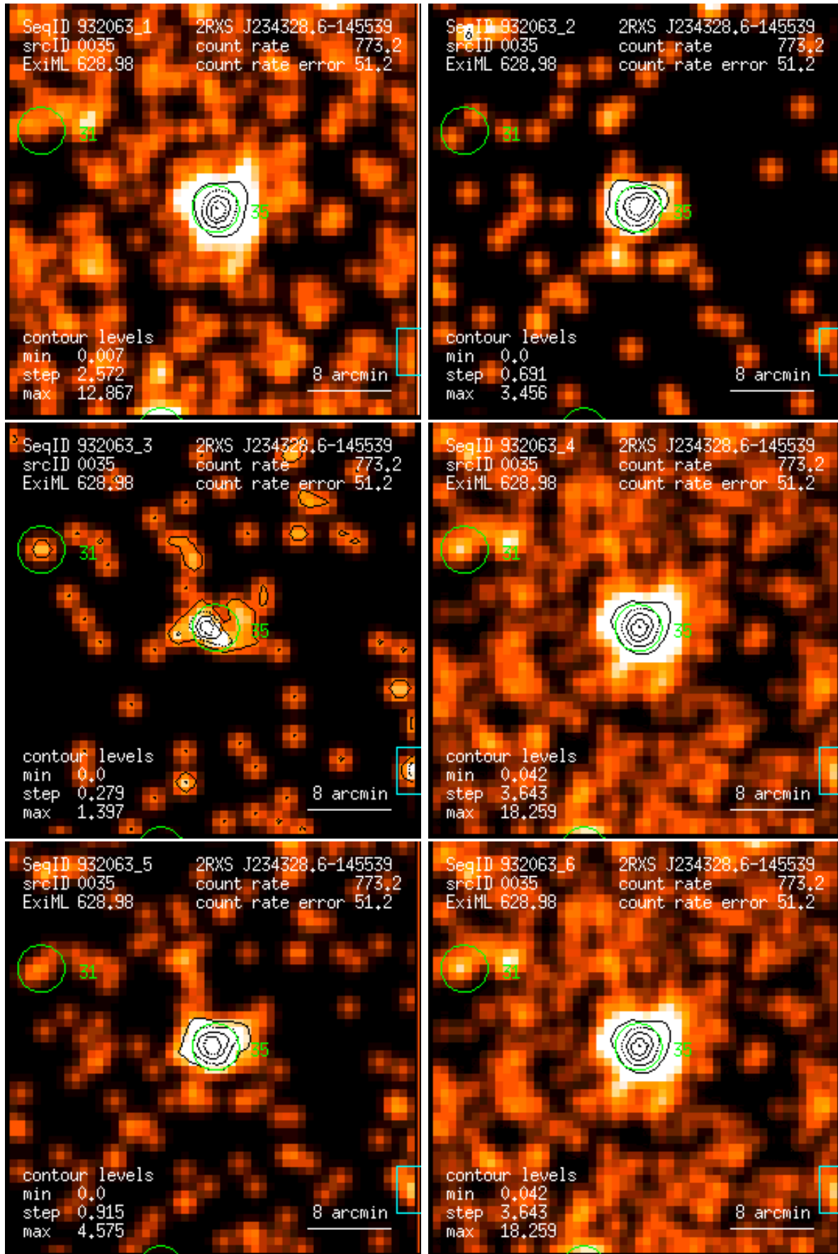
Figure 35: RASS 932063: detection 0035: band rate images, Gaussian filter: (1) PSPC channels 11 – 41, (2) 52 – 90, (3) 91 – 201, (4) 11 – 235, (5) 52 – 201, (6) 11 – 201. Broad band rates in counts/ks. Band rate contour levels in counts/ks/arcmin 2 .
