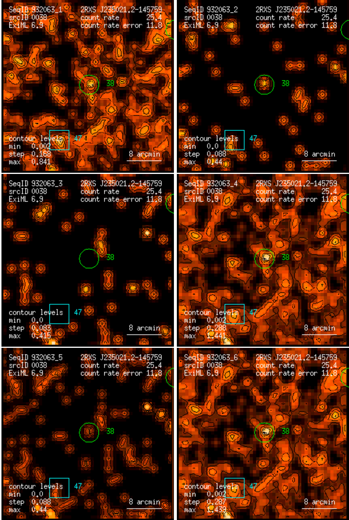
Figure 38: RASS 932063: detection 0038: band rate images, Gaussian filter: (1) PSPC channels 11 – 41, (2) 52 – 90, (3) 91 – 201, (4) 11 – 235, (5) 52 – 201, (6) 11 – 201. Broad band rates in counts/ks. Band rate contour levels in counts/ks/arcmin 2 .
