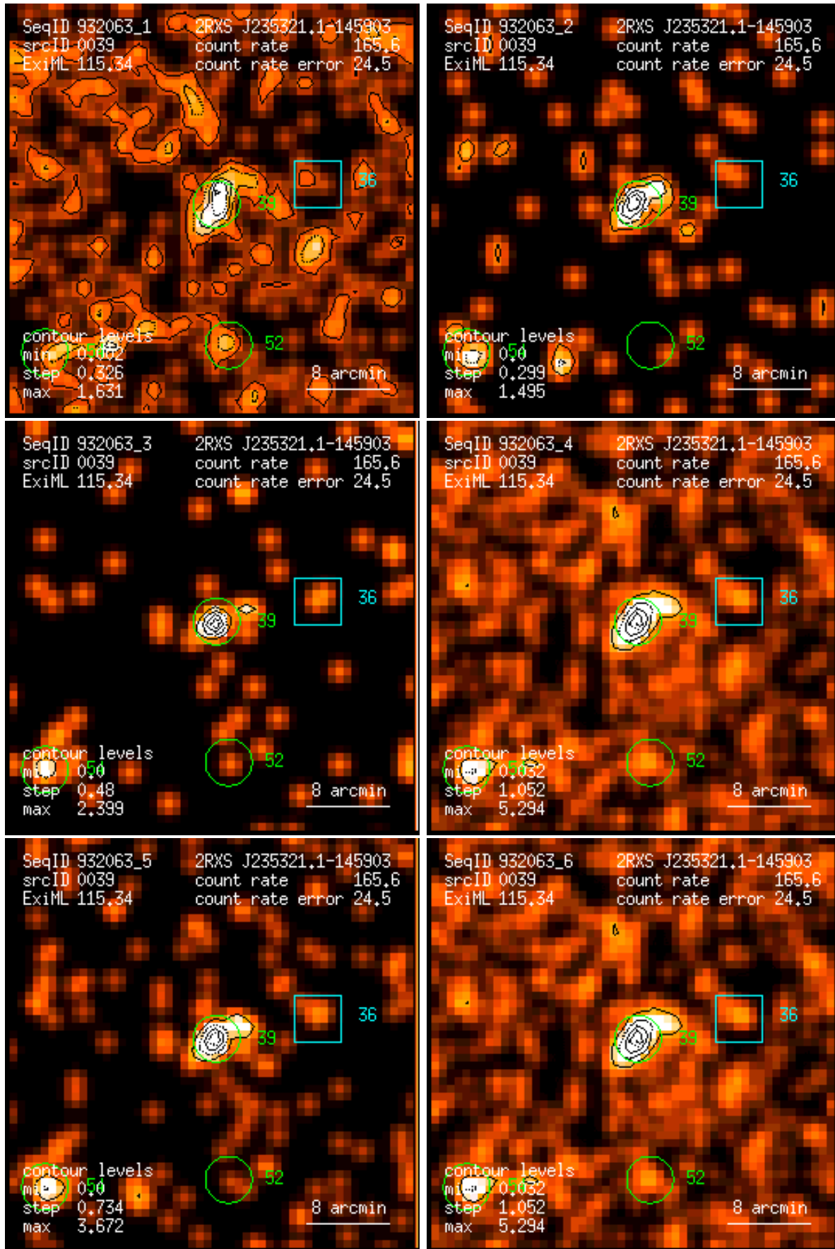
Figure 39: RASS 932063: detection 0039: band rate images, Gaussian filter: (1) PSPC channels 11 – 41, (2) 52 – 90, (3) 91 – 201, (4) 11 – 235, (5) 52 – 201, (6) 11 – 201. Broad band rates in counts/ks. Band rate contour levels in counts/ks/arcmin 2 .
