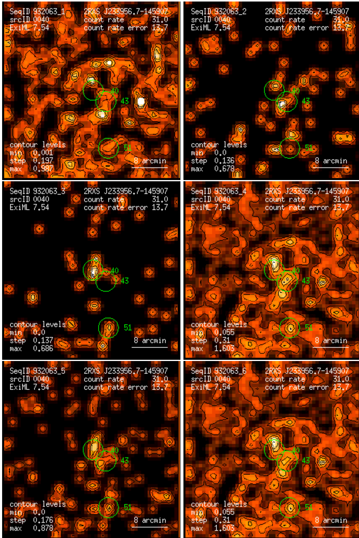
Figure 40: RASS 932063: detection 0040: band rate images, Gaussian filter: (1) PSPC channels 11 – 41, (2) 52 – 90, (3) 91 – 201, (4) 11 – 235, (5) 52 – 201, (6) 11 – 201. Broad band rates in counts/ks. Band rate contour levels in counts/ks/arcmin 2 .
