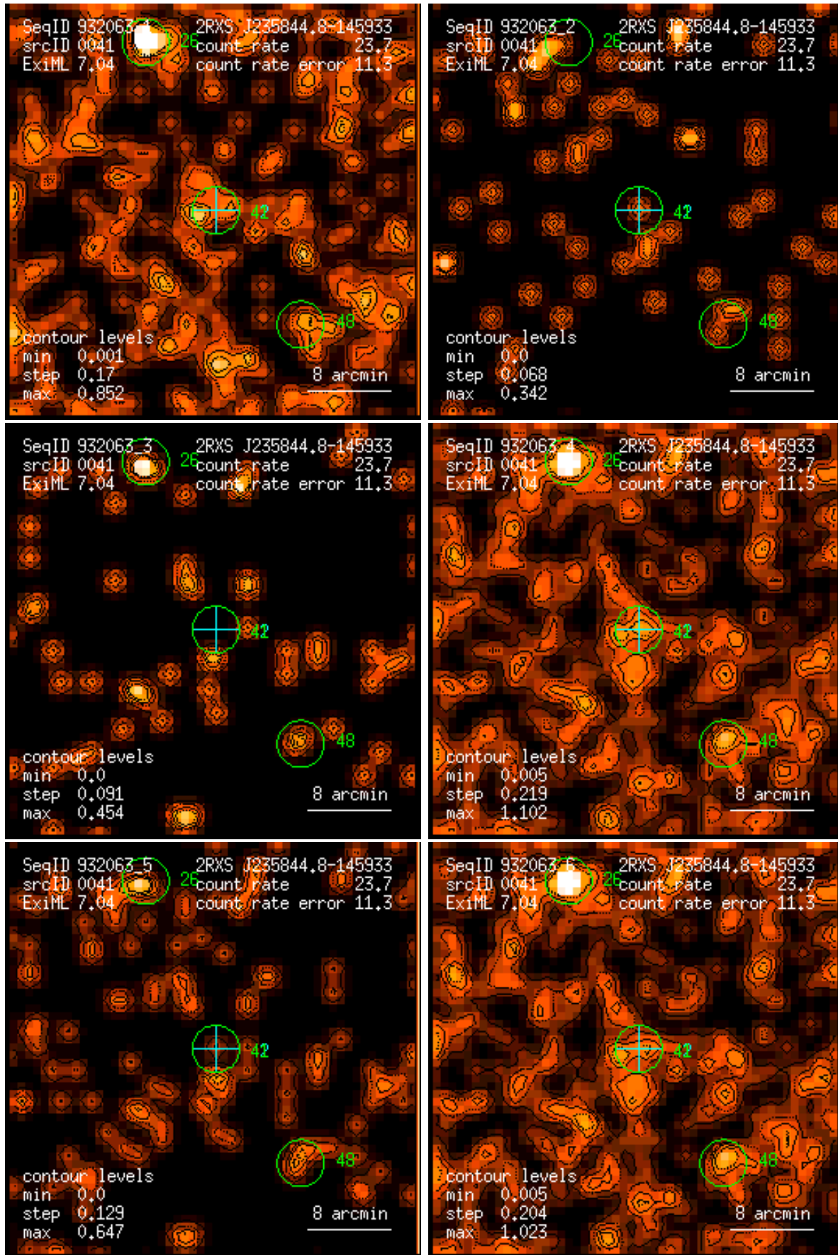
Figure 41: RASS 932063: detection 0041: band rate images, Gaussian filter: (1) PSPC channels 11 – 41, (2) 52 – 90, (3) 91 – 201, (4) 11 – 235, (5) 52 – 201, (6) 11 – 201. Broad band rates in counts/ks. Band rate contour levels in counts/ks/arcmin 2 .
