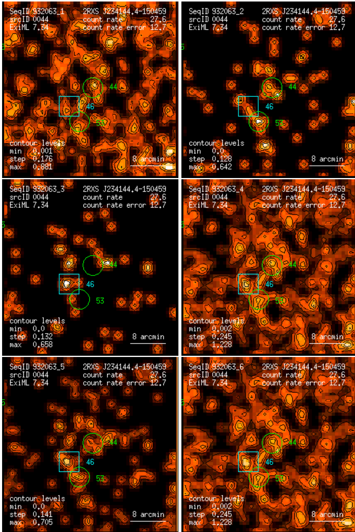
Figure 44: RASS 932063: detection 0044: band rate images, Gaussian filter: (1) PSPC channels 11 – 41, (2) 52 – 90, (3) 91 – 201, (4) 11 – 235, (5) 52 – 201, (6) 11 – 201. Broad band rates in counts/ks. Band rate contour levels in counts/ks/arcmin 2 .
