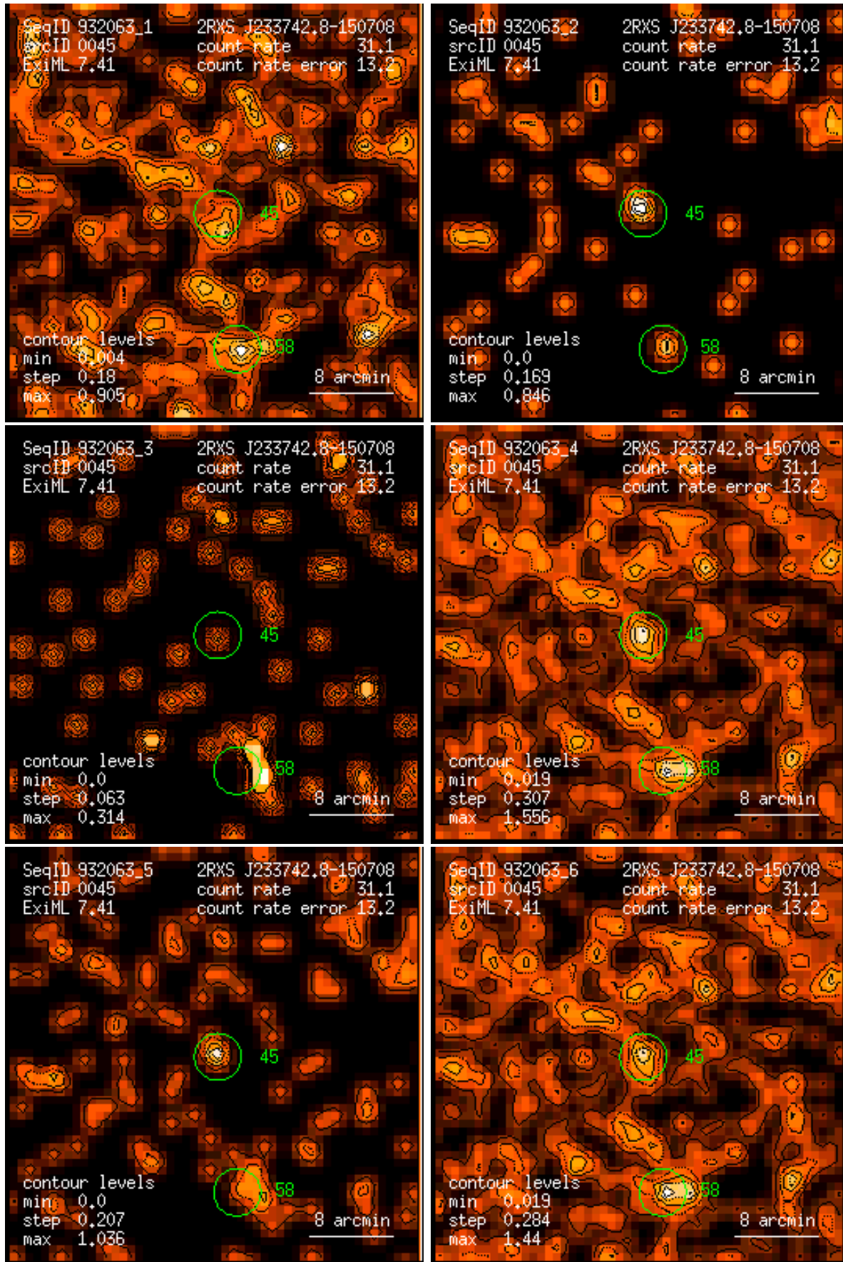
Figure 45: RASS 932063: detection 0045: band rate images, Gaussian filter: (1) PSPC channels 11 – 41, (2) 52 – 90, (3) 91 – 201, (4) 11 – 235, (5) 52 – 201, (6) 11 – 201. Broad band rates in counts/ks. Band rate contour levels in counts/ks/arcmin 2 .
