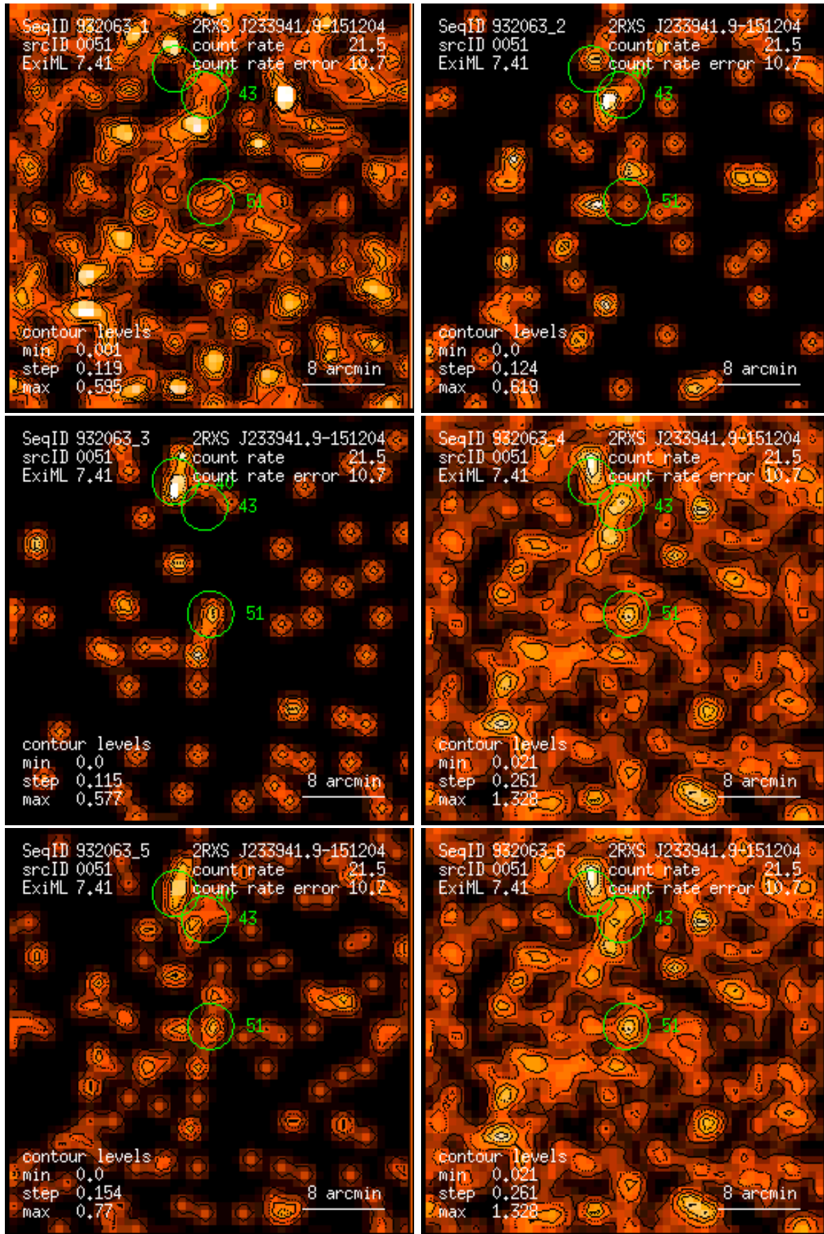
Figure 51: RASS 932063: detection 0051: band rate images, Gaussian filter: (1) PSPC channels 11 – 41, (2) 52 – 90, (3) 91 – 201, (4) 11 – 235, (5) 52 – 201, (6) 11 – 201. Broad band rates in counts/ks. Band rate contour levels in counts/ks/arcmin 2 .
