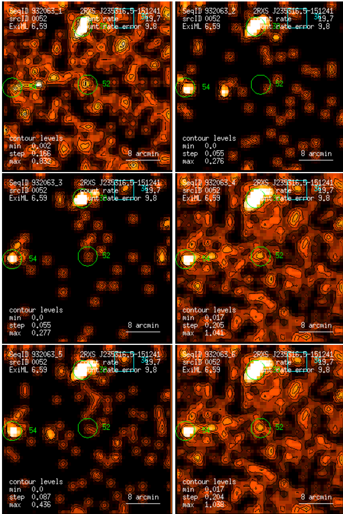
Figure 52: RASS 932063: detection 0052: band rate images, Gaussian filter: (1) PSPC channels 11 – 41, (2) 52 – 90, (3) 91 – 201, (4) 11 – 235, (5) 52 – 201, (6) 11 – 201. Broad band rates in counts/ks. Band rate contour levels in counts/ks/arcmin 2 .
