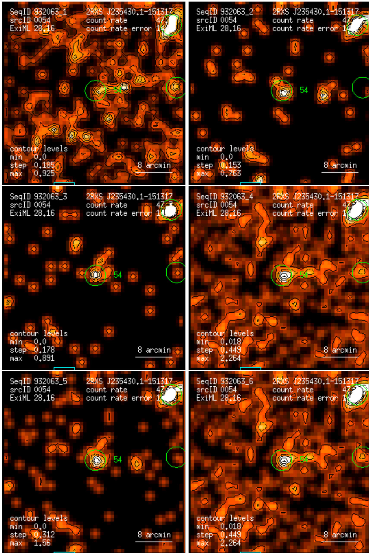
Figure 54: RASS 932063: detection 0054: band rate images, Gaussian filter: (1) PSPC channels 11 – 41, (2) 52 – 90, (3) 91 – 201, (4) 11 – 235, (5) 52 – 201, (6) 11 – 201. Broad band rates in counts/ks. Band rate contour levels in counts/ks/arcmin 2 .
