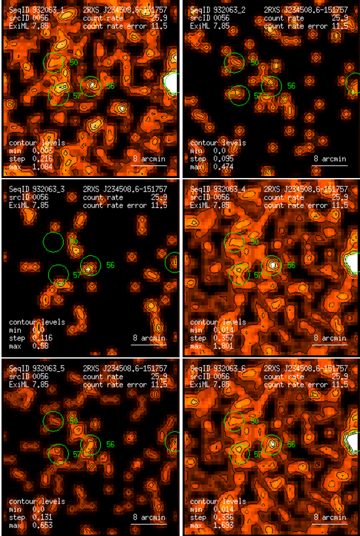
Figure 56: RASS 932063: detection 0056: band rate images, Gaussian filter: (1) PSPC channels 11 – 41, (2) 52 – 90, (3) 91 – 201, (4) 11 – 235, (5) 52 – 201, (6) 11 – 201. Broad band rates in counts/ks. Band rate contour levels in counts/ks/arcmin 2 .
