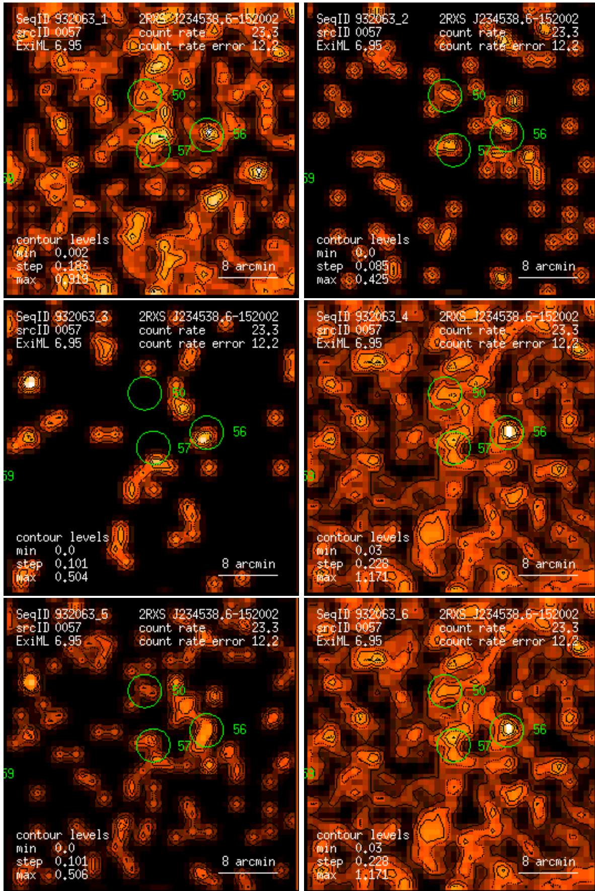
Figure 57: RASS 932063: detection 0057: band rate images, Gaussian filter: (1) PSPC channels 11 – 41, (2) 52 – 90, (3) 91 – 201, (4) 11 – 235, (5) 52 – 201, (6) 11 – 201. Broad band rates in counts/ks. Band rate contour levels in counts/ks/arcmin 2 .
