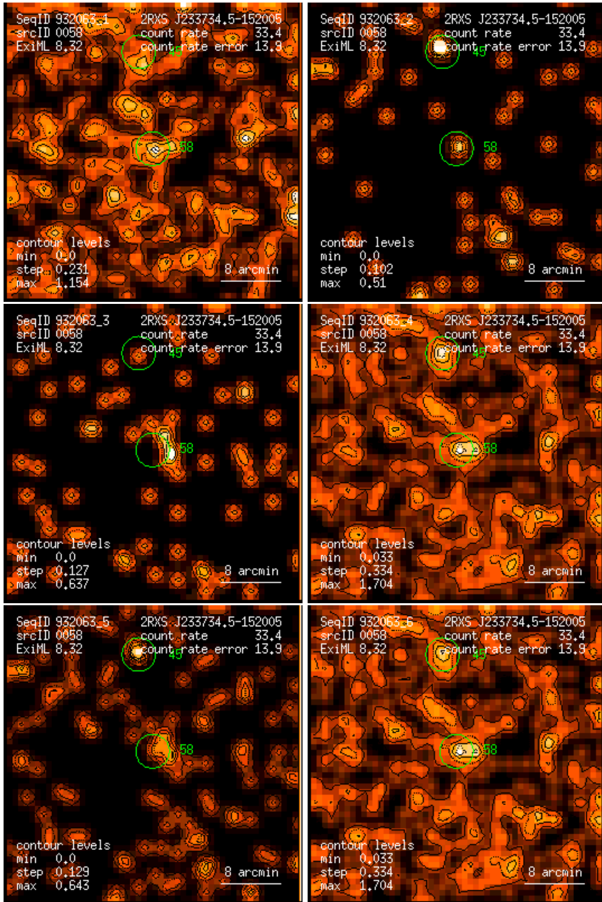
Figure 58: RASS 932063: detection 0058: band rate images, Gaussian filter: (1) PSPC channels 11 – 41, (2) 52 – 90, (3) 91 – 201, (4) 11 – 235, (5) 52 – 201, (6) 11 – 201. Broad band rates in counts/ks. Band rate contour levels in counts/ks/arcmin 2 .
