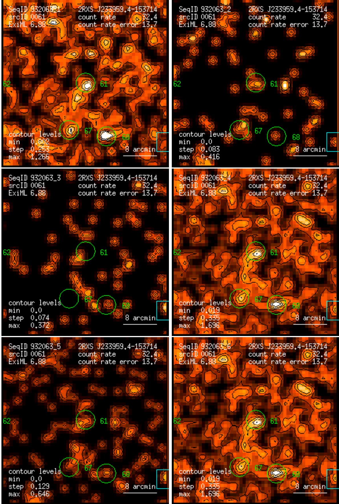
Figure 61: RASS 932063: detection 0061: band rate images, Gaussian filter: (1) PSPC channels 11 – 41, (2) 52 – 90, (3) 91 – 201, (4) 11 – 235, (5) 52 – 201, (6) 11 – 201. Broad band rates in counts/ks. Band rate contour levels in counts/ks/arcmin 2 .
