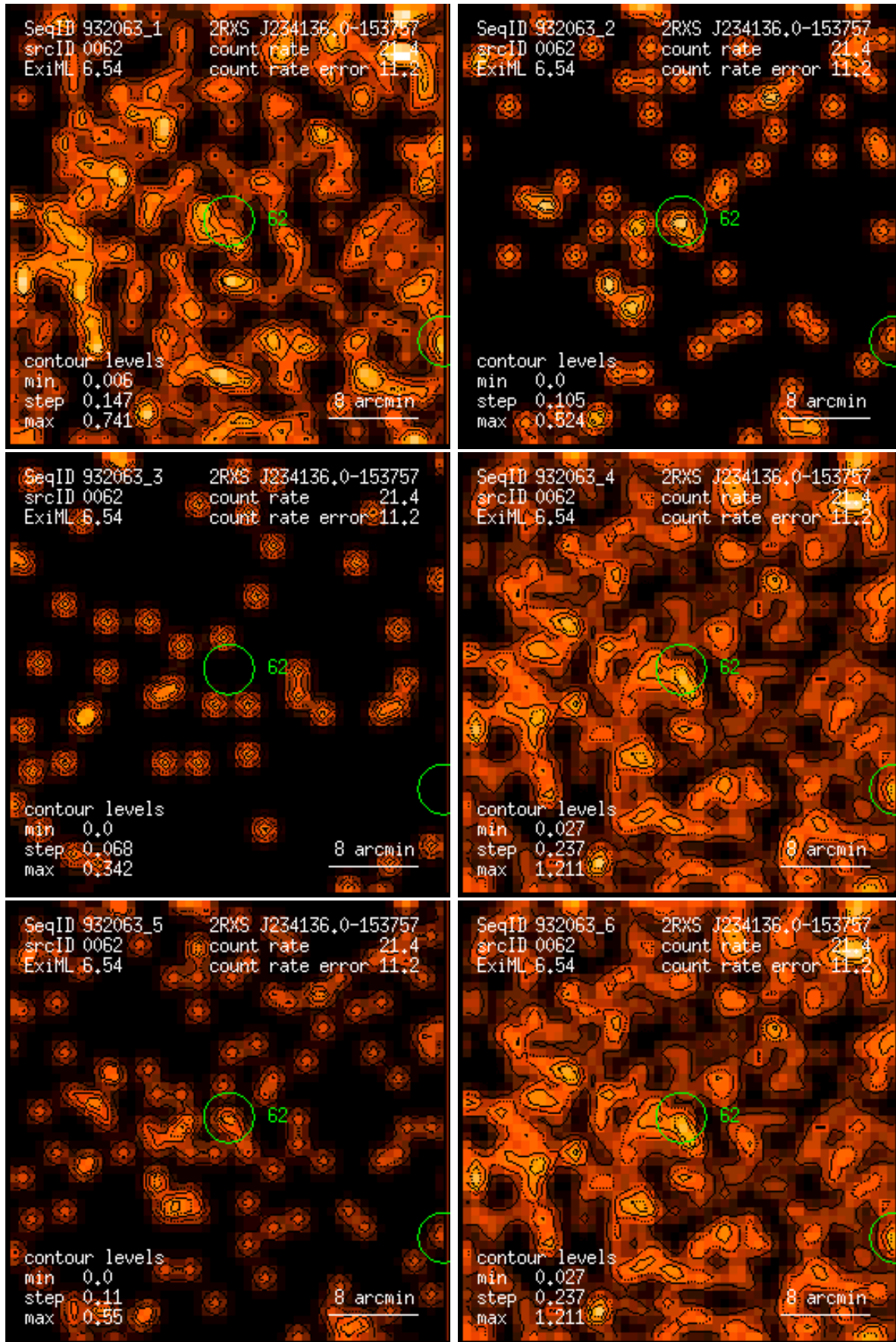
Figure 62: RASS 932063: detection 0062: band rate images, Gaussian filter: (1) PSPC channels 11 – 41, (2) 52 – 90, (3) 91 – 201, (4) 11 – 235, (5) 52 – 201, (6) 11 – 201. Broad band rates in counts/ks. Band rate contour levels in counts/ks/arcmin 2 .
