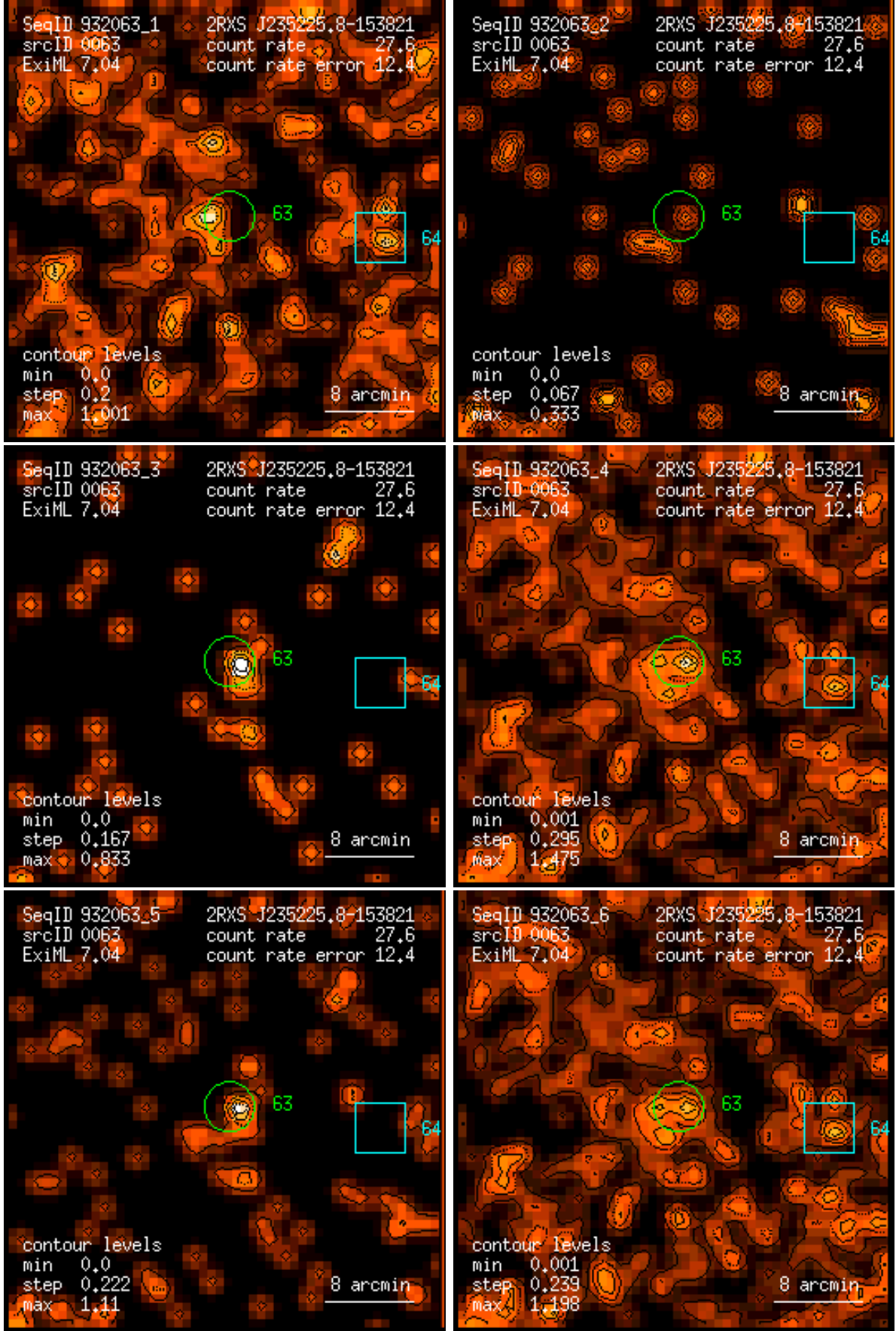
Figure 63: RASS 932063: detection 0063: band rate images, Gaussian filter: (1) PSPC channels 11 – 41, (2) 52 – 90, (3) 91 – 201, (4) 11 – 235, (5) 52 – 201, (6) 11 – 201. Broad band rates in counts/ks. Band rate contour levels in counts/ks/arcmin 2 .
