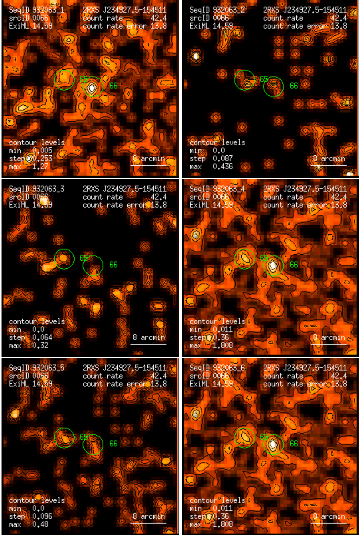
Figure 66: RASS 932063: detection 0066: band rate images, Gaussian filter: (1) PSPC channels 11 – 41, (2) 52 – 90, (3) 91 – 201, (4) 11 – 235, (5) 52 – 201, (6) 11 – 201. Broad band rates in counts/ks. Band rate contour levels in counts/ks/arcmin 2 .
