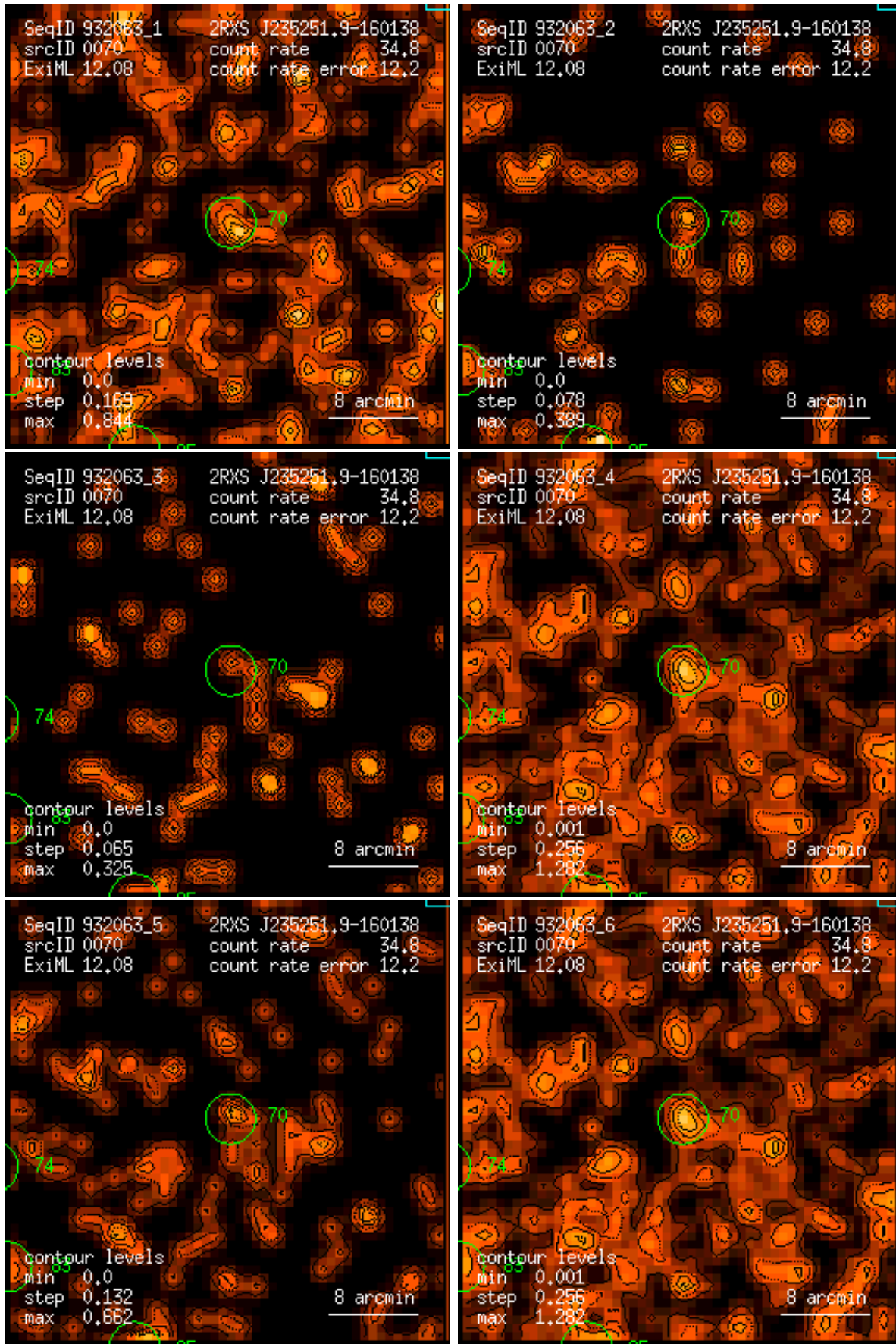
Figure 70: RASS 932063: detection 0070: band rate images, Gaussian filter: (1) PSPC channels 11 – 41, (2) 52 – 90, (3) 91 – 201, (4) 11 – 235, (5) 52 – 201, (6) 11 – 201. Broad band rates in counts/ks. Band rate contour levels in counts/ks/arcmin 2 .
