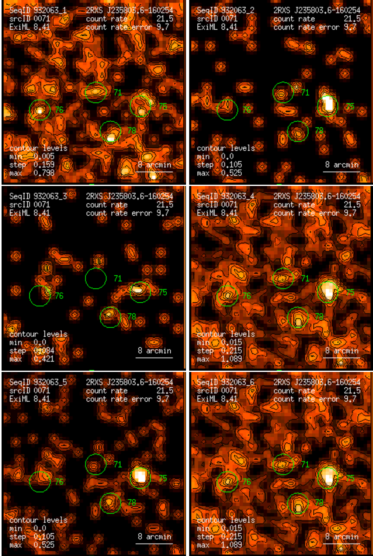
Figure 71: RASS 932063: detection 0071: band rate images, Gaussian filter: (1) PSPC channels 11 – 41, (2) 52 – 90, (3) 91 – 201, (4) 11 – 235, (5) 52 – 201, (6) 11 – 201. Broad band rates in counts/ks. Band rate contour levels in counts/ks/arcmin 2 .
