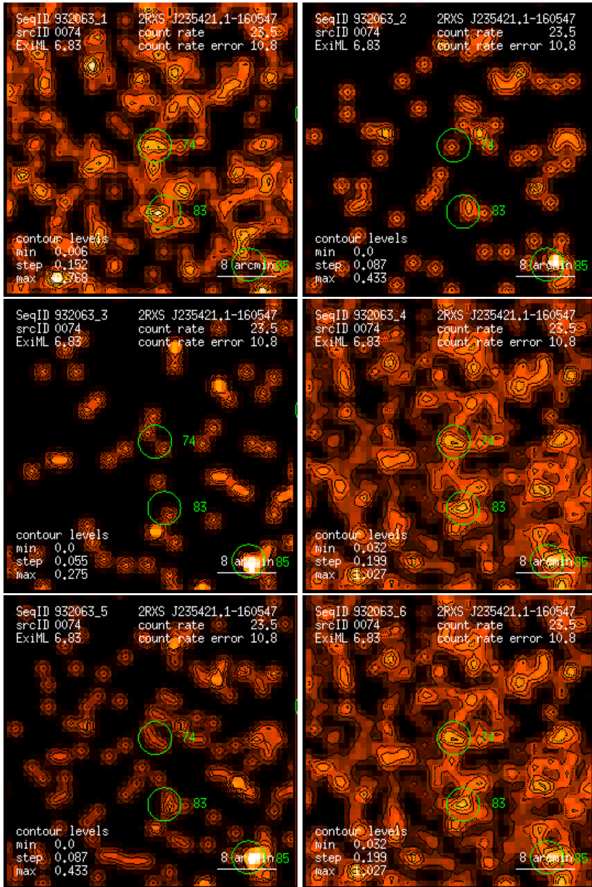
Figure 74: RASS 932063: detection 0074: band rate images, Gaussian filter: (1) PSPC channels 11 – 41, (2) 52 – 90, (3) 91 – 201, (4) 11 – 235, (5) 52 – 201, (6) 11 – 201. Broad band rates in counts/ks. Band rate contour levels in counts/ks/arcmin 2 .
