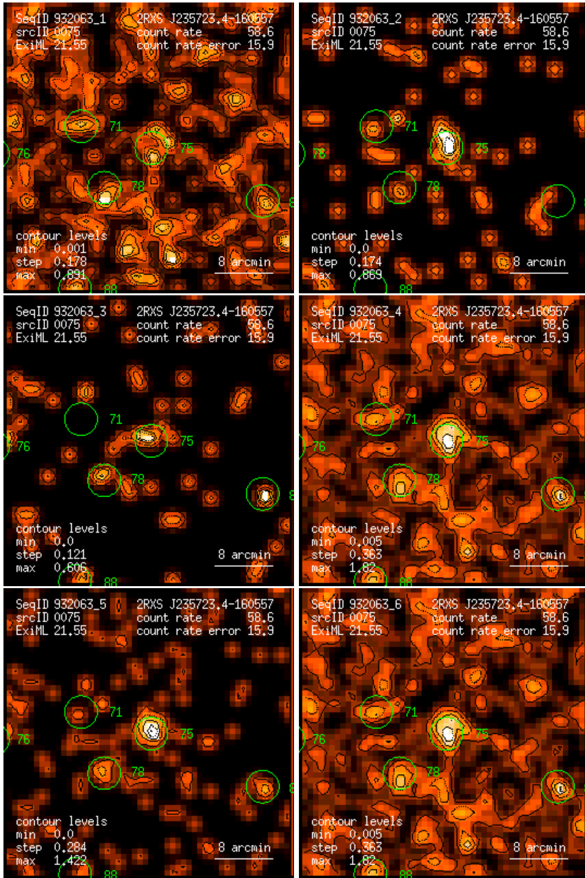
Figure 75: RASS 932063: detection 0075: band rate images, Gaussian filter: (1) PSPC channels 11 – 41, (2) 52 – 90, (3) 91 – 201, (4) 11 – 235, (5) 52 – 201, (6) 11 – 201. Broad band rates in counts/ks. Band rate contour levels in counts/ks/arcmin 2 .
