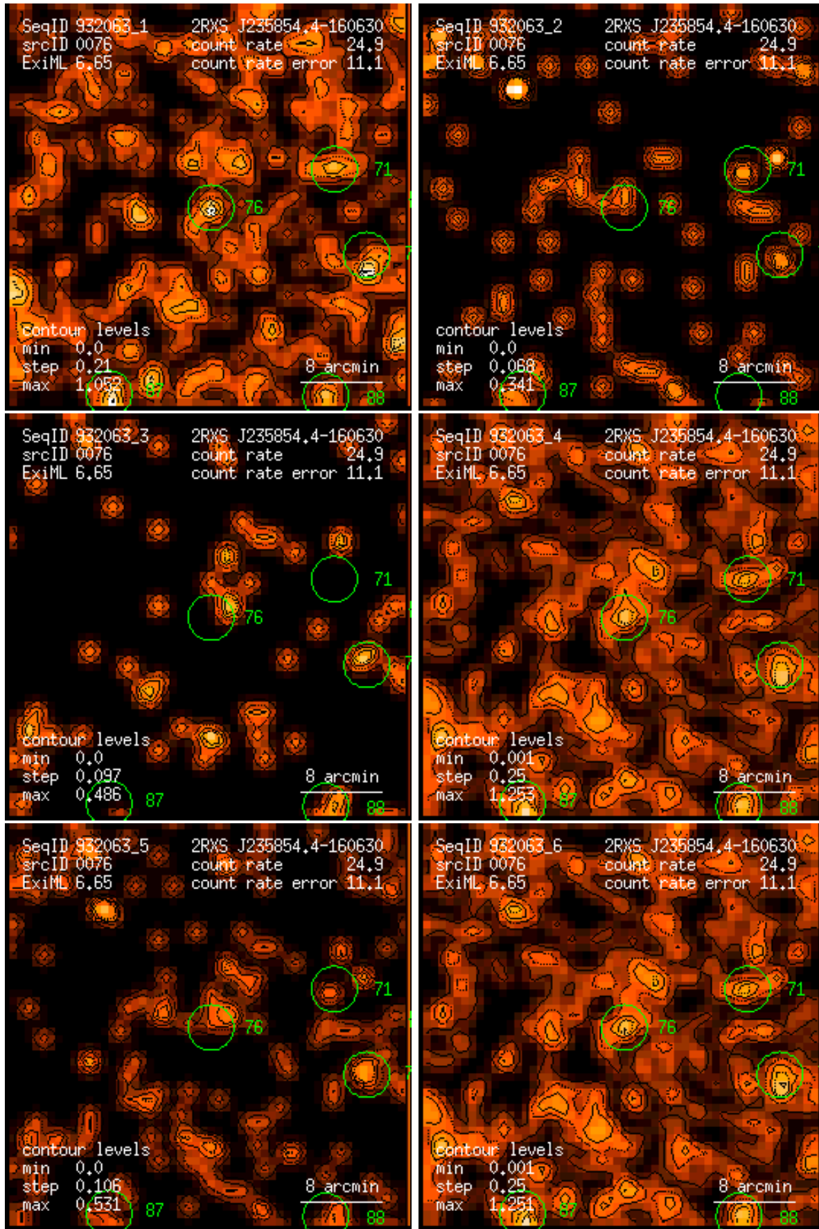
Figure 76: RASS 932063: detection 0076: band rate images, Gaussian filter: (1) PSPC channels 11 – 41, (2) 52 – 90, (3) 91 – 201, (4) 11 – 235, (5) 52 – 201, (6) 11 – 201. Broad band rates in counts/ks. Band rate contour levels in counts/ks/arcmin 2 .
