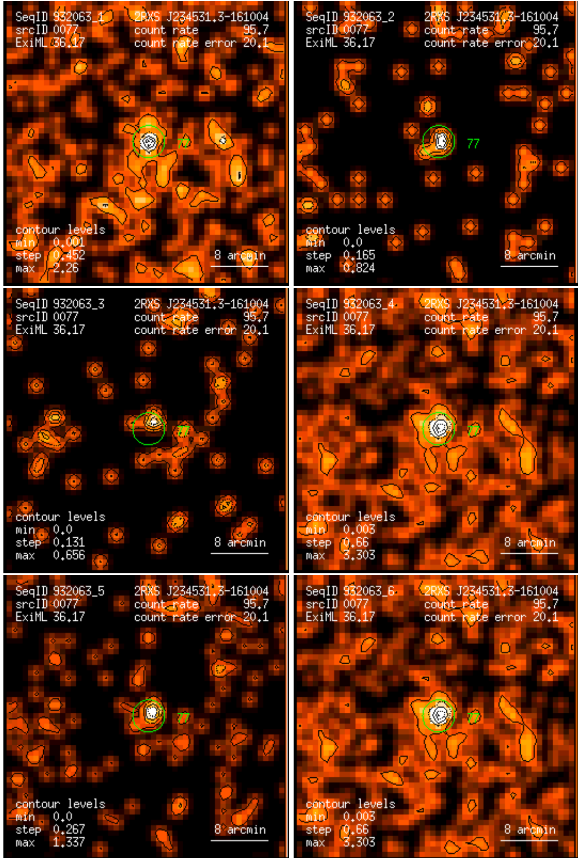
Figure 77: RASS 932063: detection 0077: band rate images, Gaussian filter: (1) PSPC channels 11 – 41, (2) 52 – 90, (3) 91 – 201, (4) 11 – 235, (5) 52 – 201, (6) 11 – 201. Broad band rates in counts/ks. Band rate contour levels in counts/ks/arcmin 2 .
