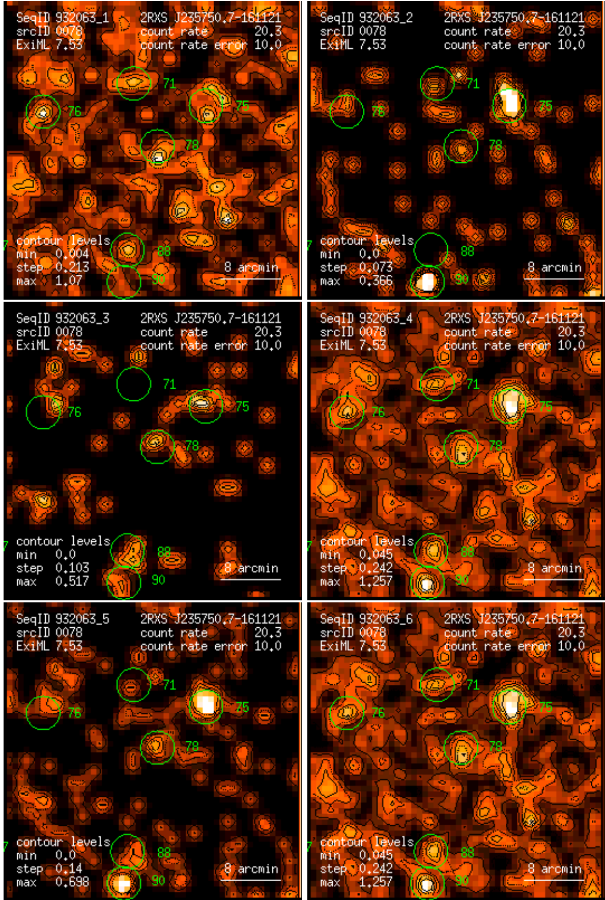
Figure 78: RASS 932063: detection 0078: band rate images, Gaussian filter: (1) PSPC channels 11 – 41, (2) 52 – 90, (3) 91 – 201, (4) 11 – 235, (5) 52 – 201, (6) 11 – 201. Broad band rates in counts/ks. Band rate contour levels in counts/ks/arcmin 2 .
