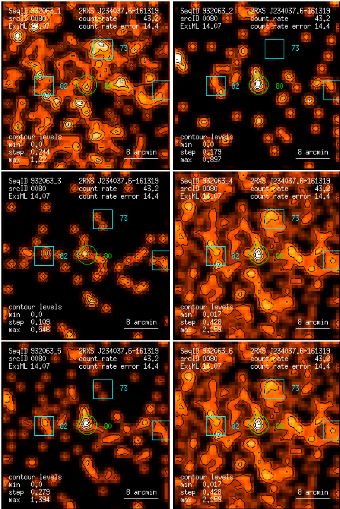
Figure 80: RASS 932063: detection 0080: band rate images, Gaussian filter: (1) PSPC channels 11 – 41, (2) 52 – 90, (3) 91 – 201, (4) 11 – 235, (5) 52 – 201, (6) 11 – 201. Broad band rates in counts/ks. Band rate contour levels in counts/ks/arcmin 2 .
