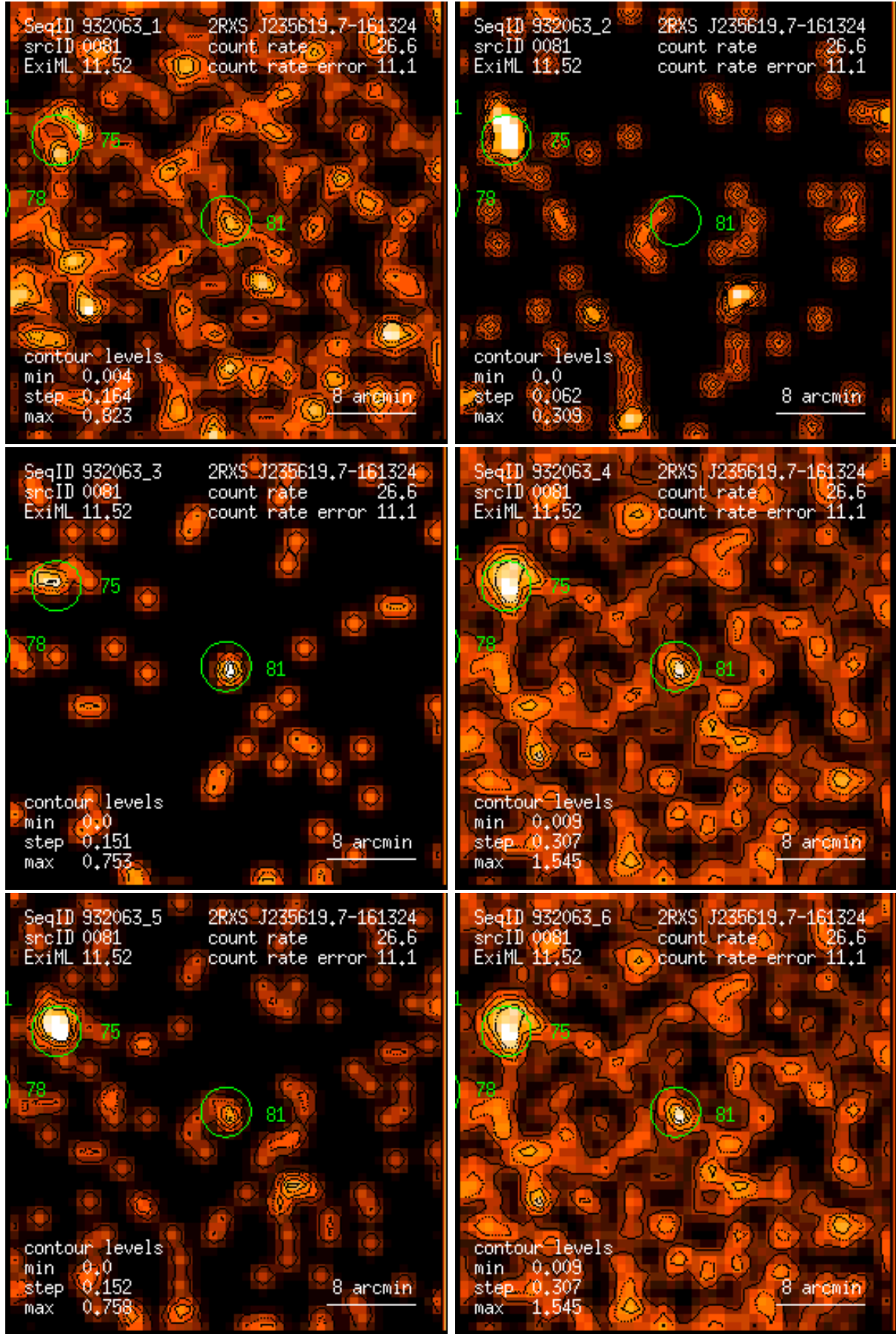
Figure 81: RASS 932063: detection 0081: band rate images, Gaussian filter: (1) PSPC channels 11 – 41, (2) 52 – 90, (3) 91 – 201, (4) 11 – 235, (5) 52 – 201, (6) 11 – 201. Broad band rates in counts/ks. Band rate contour levels in counts/ks/arcmin 2 .
