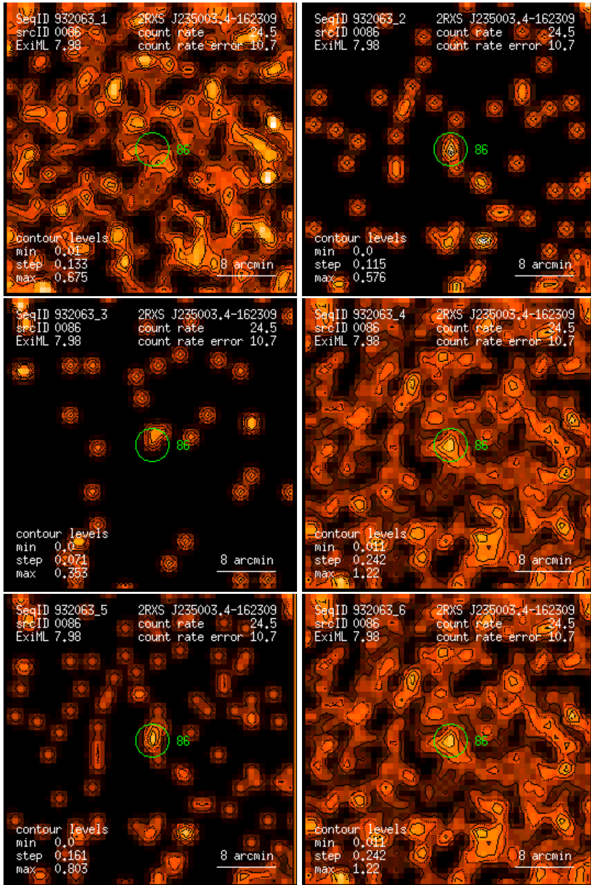
Figure 86: RASS 932063: detection 0086: band rate images, Gaussian filter: (1) PSPC channels 11 – 41, (2) 52 – 90, (3) 91 – 201, (4) 11 – 235, (5) 52 – 201, (6) 11 – 201. Broad band rates in counts/ks. Band rate contour levels in counts/ks/arcmin 2 .
