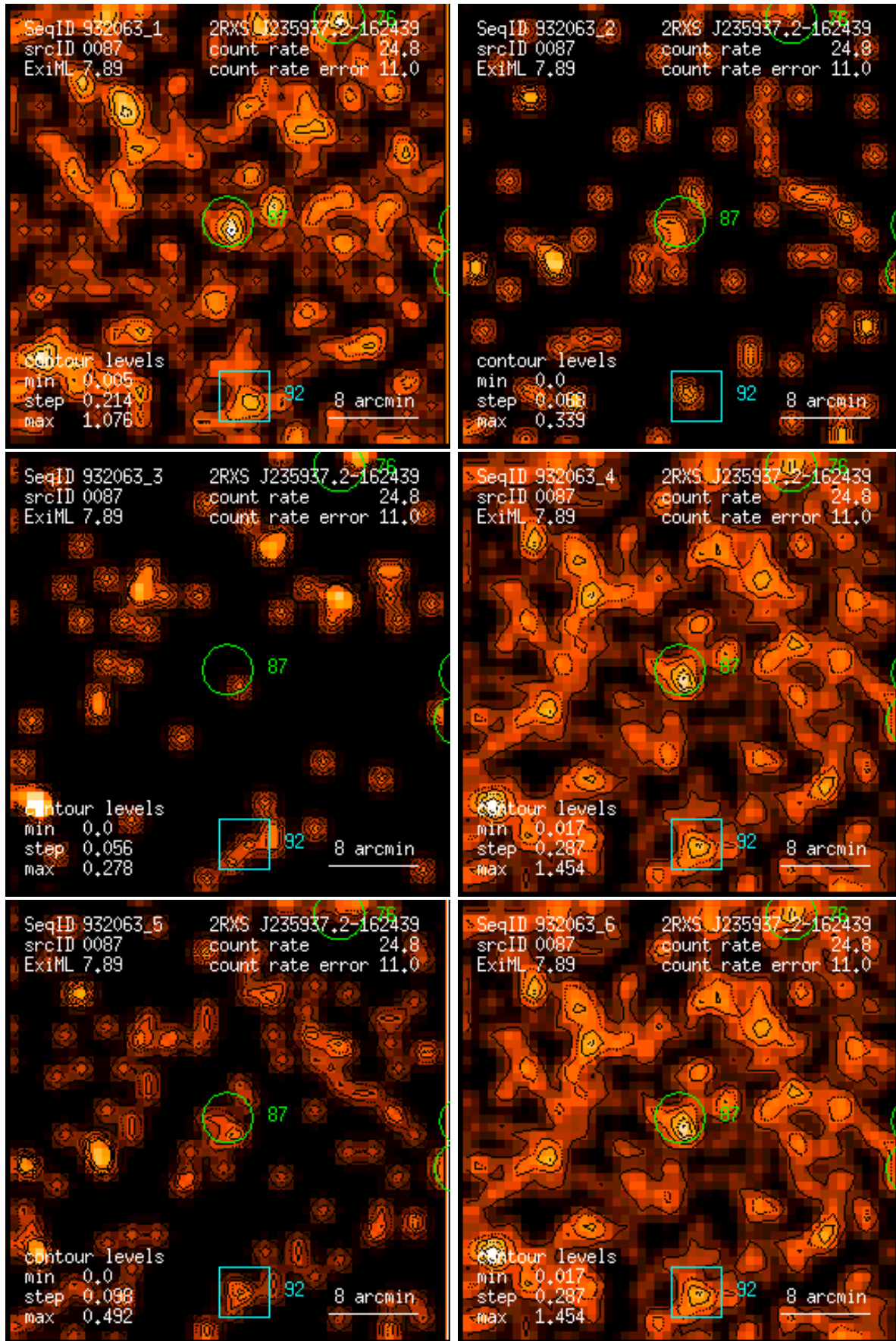
Figure 87: RASS 932063: detection 0087: band rate images, Gaussian filter: (1) PSPC channels 11 – 41, (2) 52 – 90, (3) 91 – 201, (4) 11 – 235, (5) 52 – 201, (6) 11 – 201. Broad band rates in counts/ks. Band rate contour levels in counts/ks/arcmin 2 .
