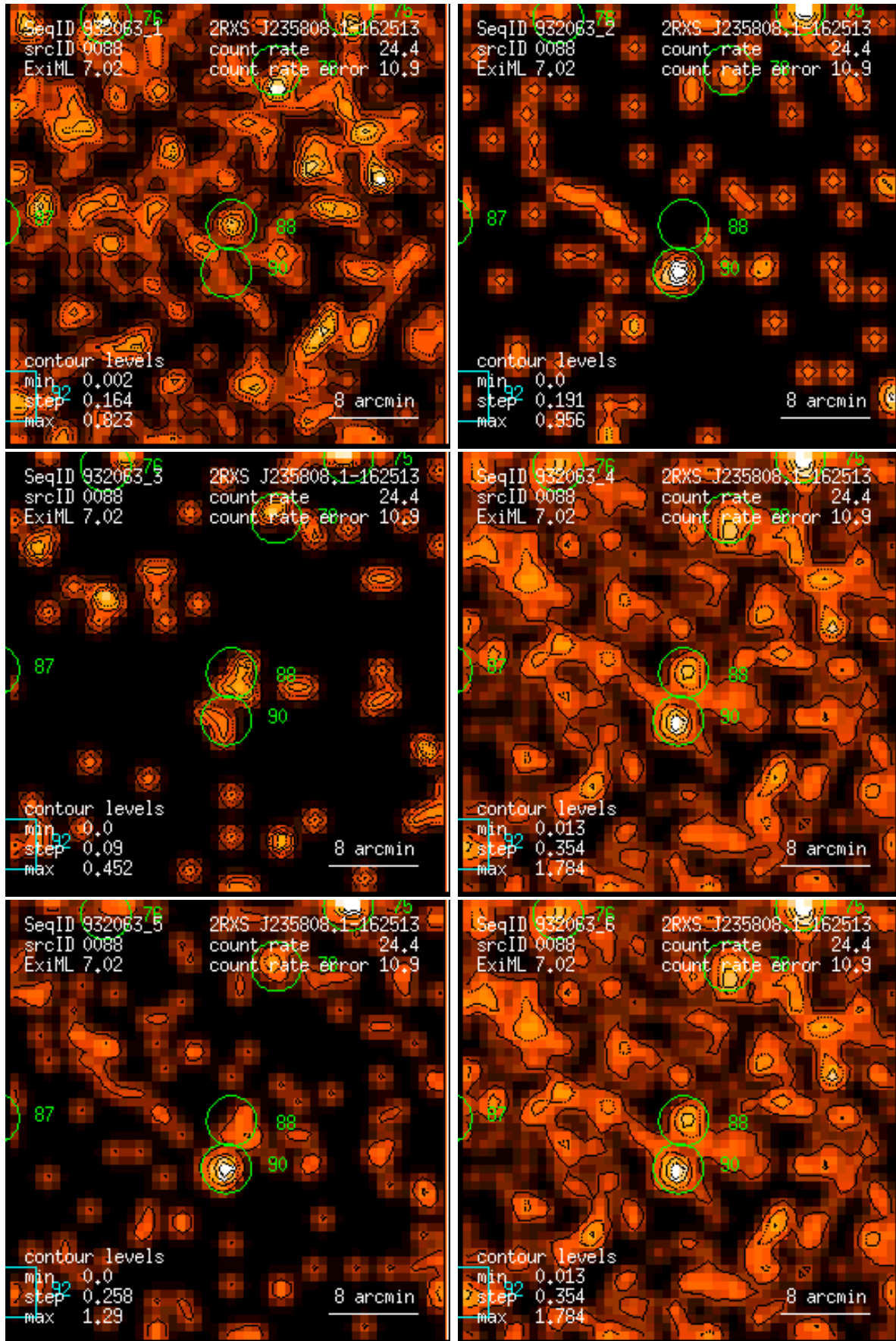
Figure 88: RASS 932063: detection 0088: band rate images, Gaussian filter: (1) PSPC channels 11 – 41, (2) 52 – 90, (3) 91 – 201, (4) 11 – 235, (5) 52 – 201, (6) 11 – 201. Broad band rates in counts/ks. Band rate contour levels in counts/ks/arcmin 2 .
