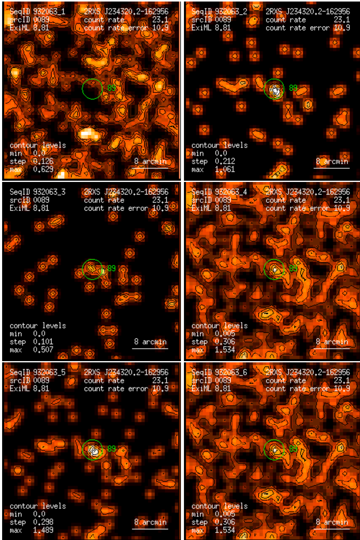
Figure 89: RASS 932063: detection 0089: band rate images, Gaussian filter: (1) PSPC channels 11 – 41, (2) 52 – 90, (3) 91 – 201, (4) 11 – 235, (5) 52 – 201, (6) 11 – 201. Broad band rates in counts/ks. Band rate contour levels in counts/ks/arcmin 2 .
