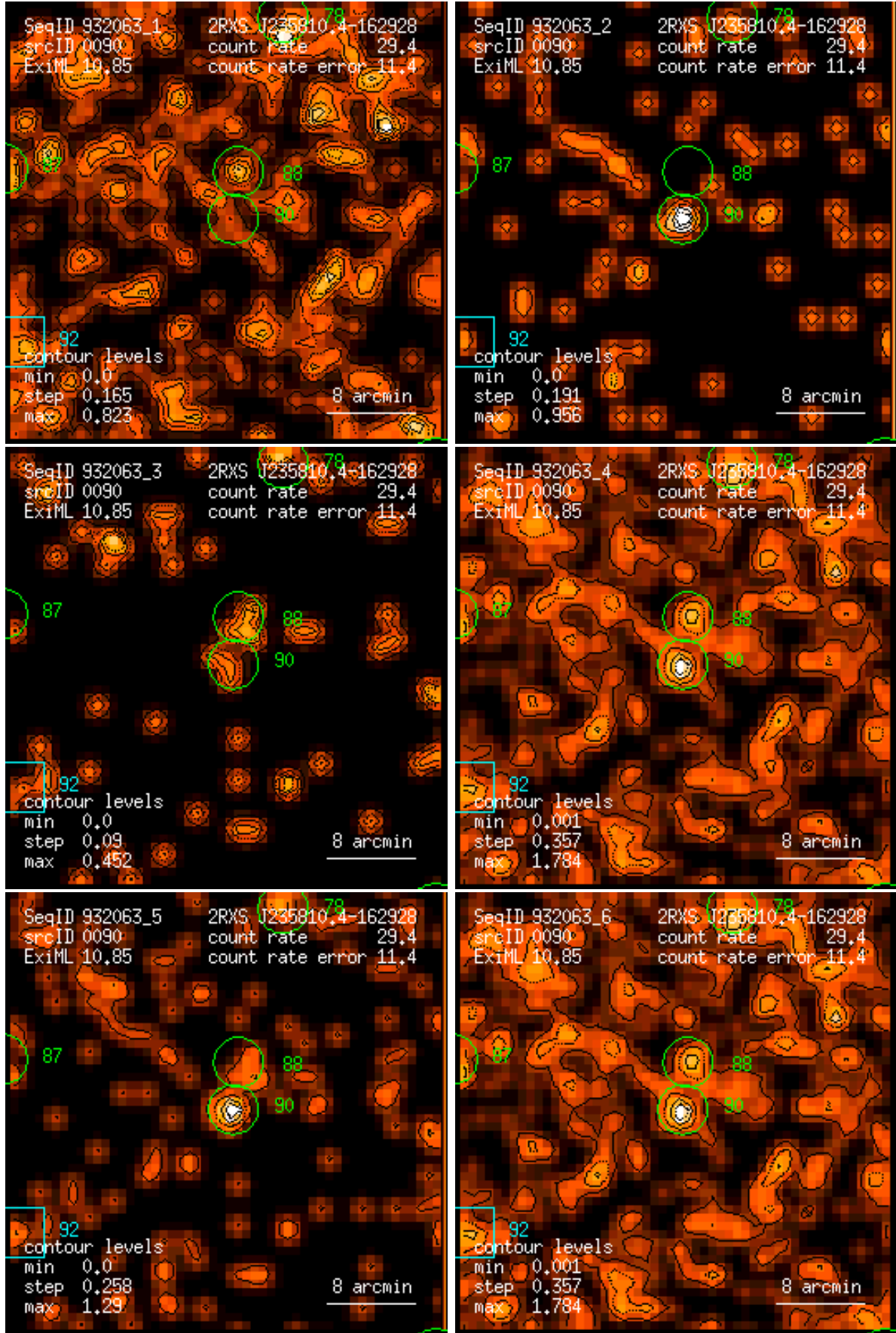
Figure 90: RASS 932063: detection 0090: band rate images, Gaussian filter: (1) PSPC channels 11 – 41, (2) 52 – 90, (3) 91 – 201, (4) 11 – 235, (5) 52 – 201, (6) 11 – 201. Broad band rates in counts/ks. Band rate contour levels in counts/ks/arcmin 2 .
