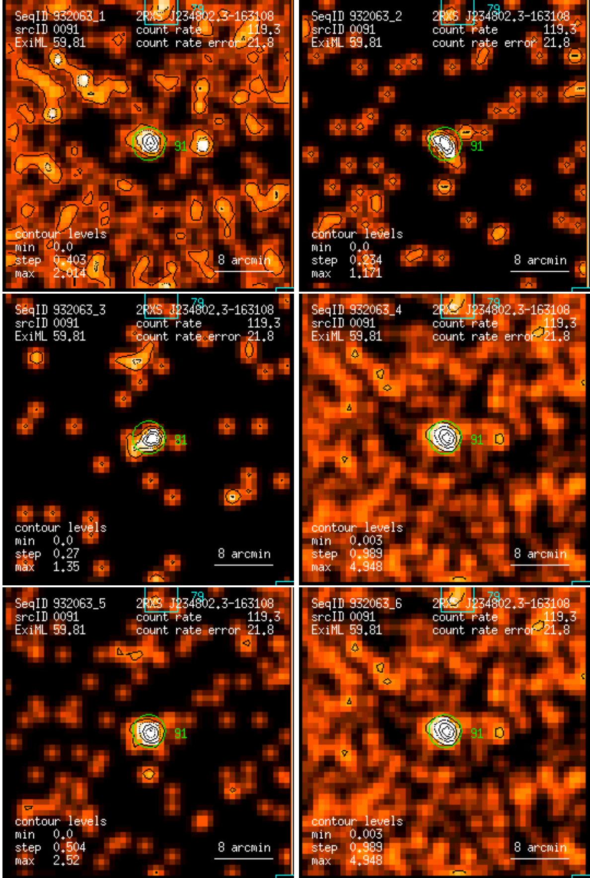
Figure 91: RASS 932063: detection 0091: band rate images, Gaussian filter: (1) PSPC channels 11 – 41, (2) 52 – 90, (3) 91 – 201, (4) 11 – 235, (5) 52 – 201, (6) 11 – 201. Broad band rates in counts/ks. Band rate contour levels in counts/ks/arcmin 2 .
