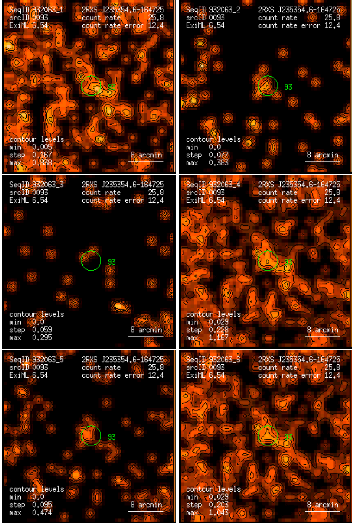
Figure 93: RASS 932063: detection 0093: band rate images, Gaussian filter: (1) PSPC channels 11 – 41, (2) 52 – 90, (3) 91 – 201, (4) 11 – 235, (5) 52 – 201, (6) 11 – 201. Broad band rates in counts/ks. Band rate contour levels in counts/ks/arcmin 2 .
