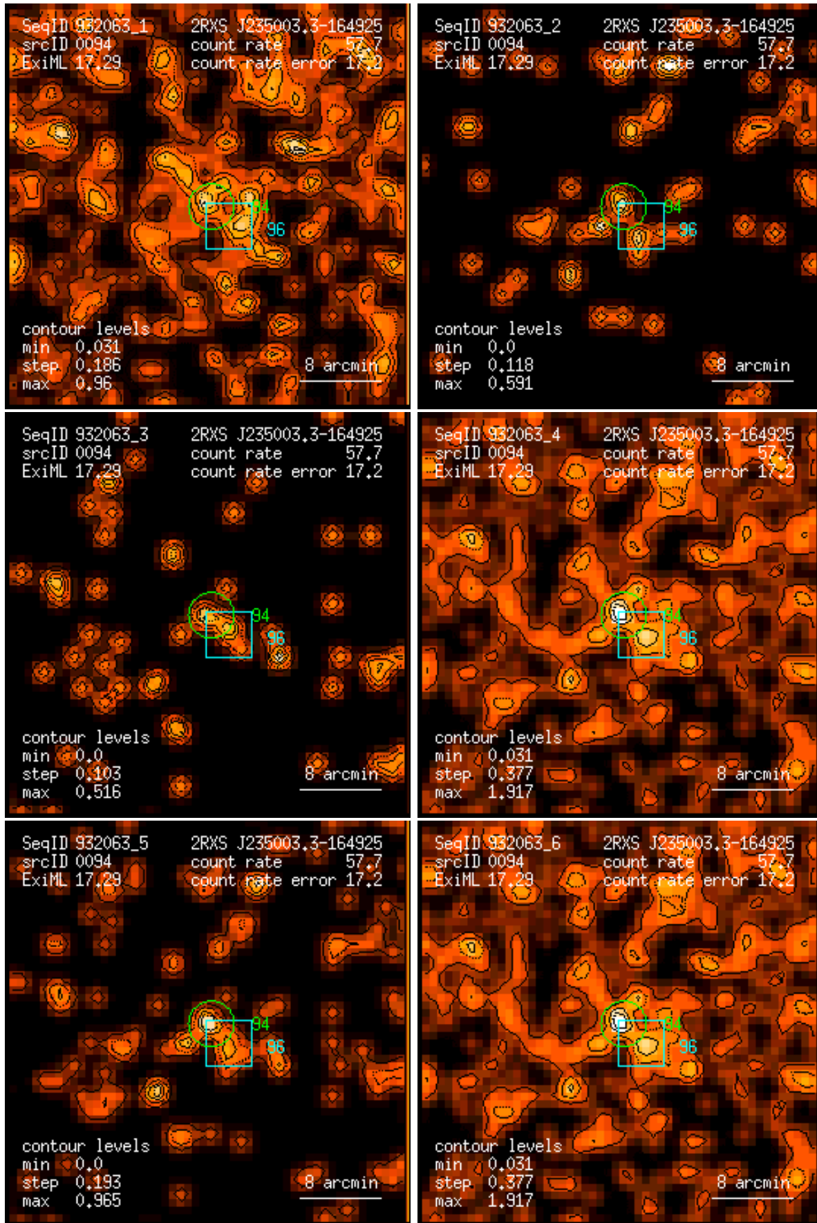
Figure 94: RASS 932063: detection 0094: band rate images, Gaussian filter: (1) PSPC channels 11 – 41, (2) 52 – 90, (3) 91 – 201, (4) 11 – 235, (5) 52 – 201, (6) 11 – 201. Broad band rates in counts/ks. Band rate contour levels in counts/ks/arcmin 2 .
