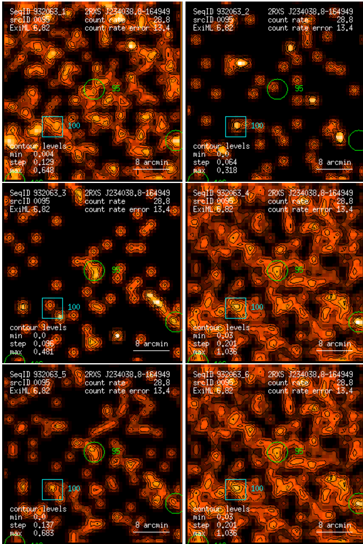
Figure 95: RASS 932063: detection 0095: band rate images, Gaussian filter: (1) PSPC channels 11 – 41, (2) 52 – 90, (3) 91 – 201, (4) 11 – 235, (5) 52 – 201, (6) 11 – 201. Broad band rates in counts/ks. Band rate contour levels in counts/ks/arcmin 2 .
