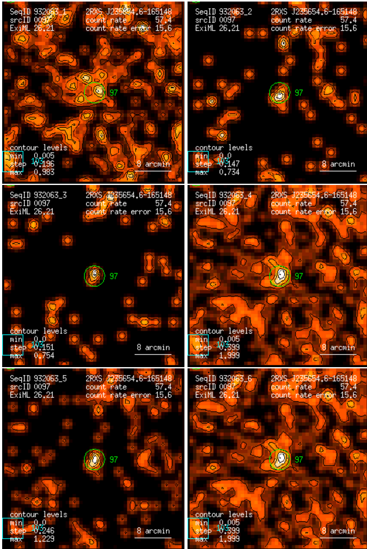
Figure 97: RASS 932063: detection 0097: band rate images, Gaussian filter: (1) PSPC channels 11 – 41, (2) 52 – 90, (3) 91 – 201, (4) 11 – 235, (5) 52 – 201, (6) 11 – 201. Broad band rates in counts/ks. Band rate contour levels in counts/ks/arcmin 2 .
