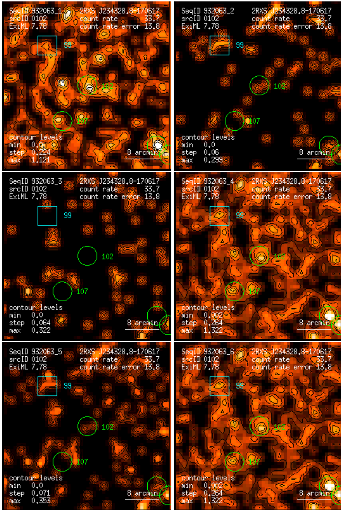
Figure 102: RASS 932063: detection 0102: band rate images, Gaussian filter: (1) PSPC channels 11 – 41, (2) 52 – 90, (3) 91 – 201, (4) 11 – 235, (5) 52 – 201, (6) 11 – 201. Broad band rates in counts/ks. Band rate contour levels in counts/ks/arcmin 2 .
