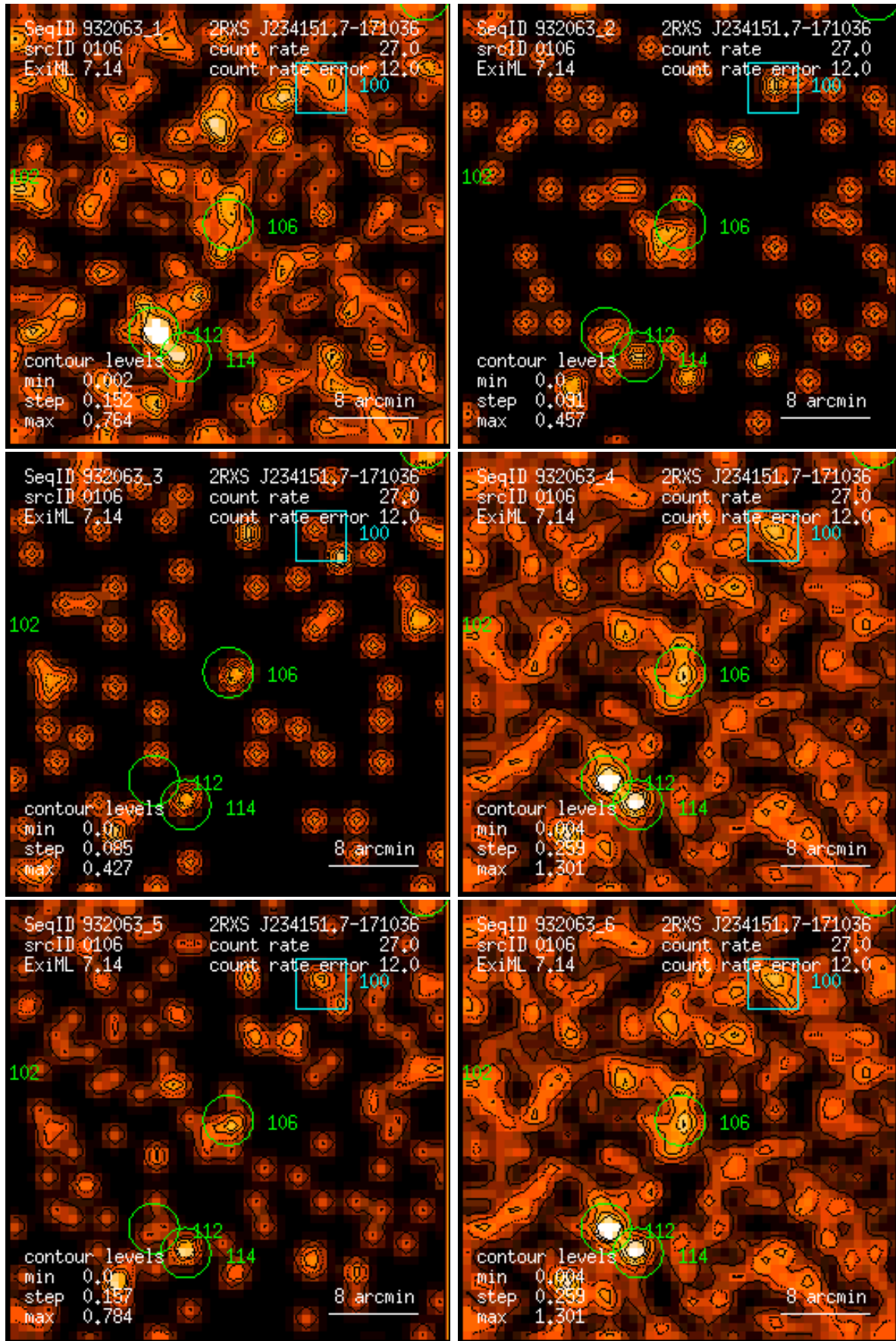
Figure 106: RASS 932063: detection 0106: band rate images, Gaussian filter: (1) PSPC channels 11 – 41, (2) 52 – 90, (3) 91 – 201, (4) 11 – 235, (5) 52 – 201, (6) 11 – 201. Broad band rates in counts/ks. Band rate contour levels in counts/ks/arcmin 2 .
