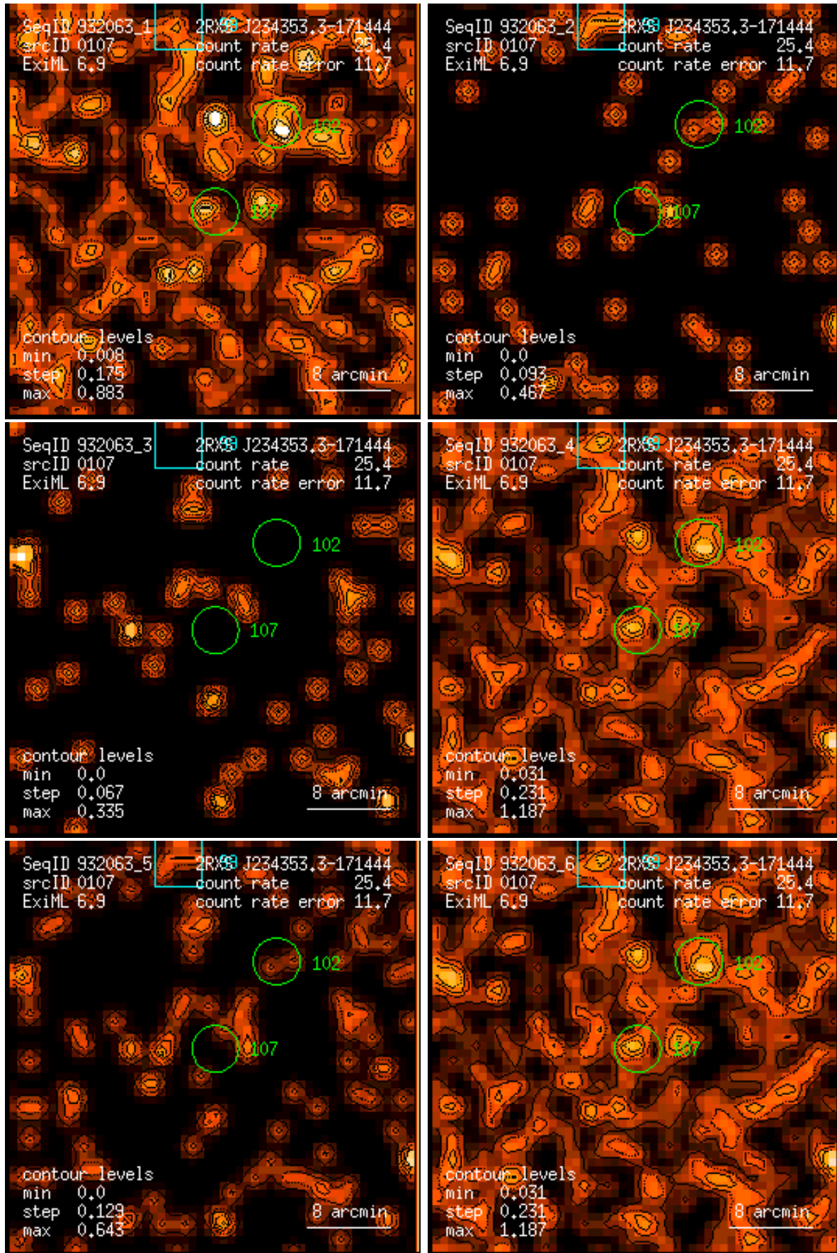
Figure 107: RASS 932063: detection 0107: band rate images, Gaussian filter: (1) PSPC channels 11 – 41, (2) 52 – 90, (3) 91 – 201, (4) 11 – 235, (5) 52 – 201, (6) 11 – 201. Broad band rates in counts/ks. Band rate contour levels in counts/ks/arcmin 2 .
