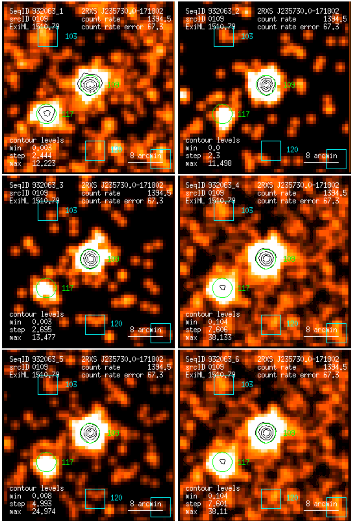
Figure 109: RASS 932063: detection 0109: band rate images, Gaussian filter: (1) PSPC channels 11 – 41, (2) 52 – 90, (3) 91 – 201, (4) 11 – 235, (5) 52 – 201, (6) 11 – 201. Broad band rates in counts/ks. Band rate contour levels in counts/ks/arcmin 2 .
