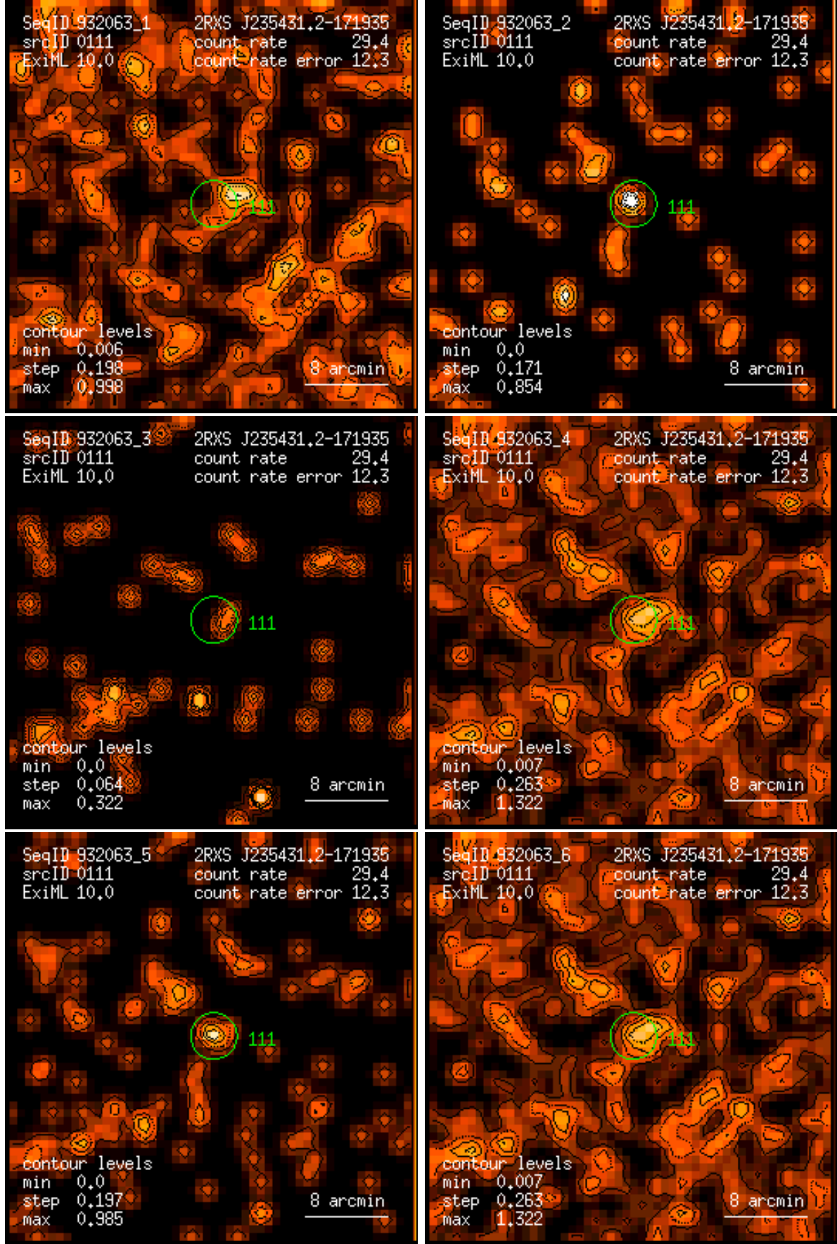
Figure 111: RASS 932063: detection 0111: band rate images, Gaussian filter: (1) PSPC channels 11 – 41, (2) 52 – 90, (3) 91 – 201, (4) 11 – 235, (5) 52 – 201, (6) 11 – 201. Broad band rates in counts/ks. Band rate contour levels in counts/ks/arcmin 2 .
