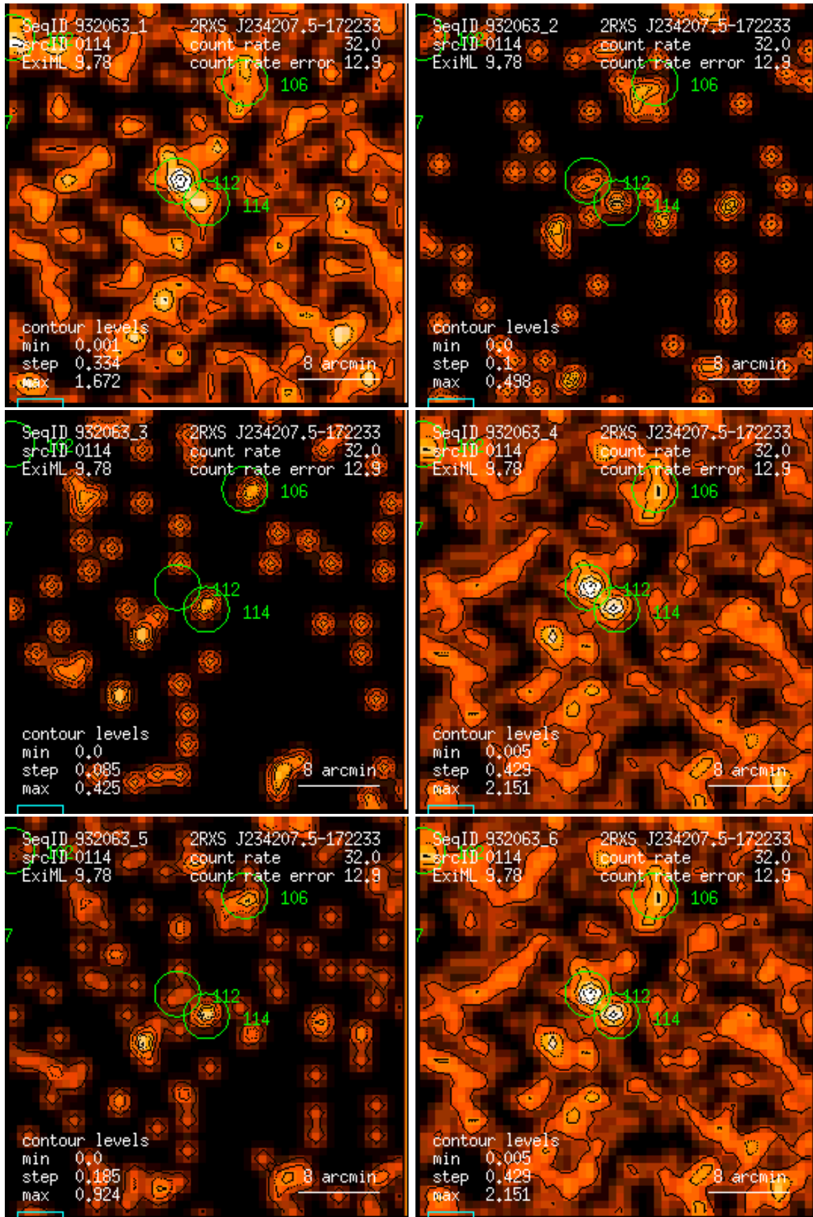
Figure 114: RASS 932063: detection 0114: band rate images, Gaussian filter: (1) PSPC channels 11 – 41, (2) 52 – 90, (3) 91 – 201, (4) 11 – 235, (5) 52 – 201, (6) 11 – 201. Broad band rates in counts/ks. Band rate contour levels in counts/ks/arcmin 2 .
