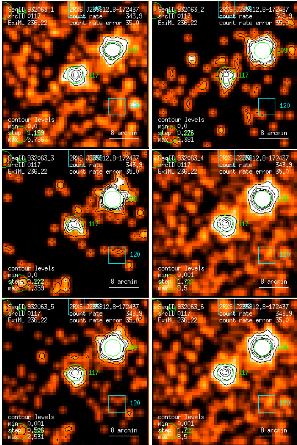
Figure 117: RASS 932063: detection 0117: band rate images, Gaussian filter: (1) PSPC channels 11 – 41, (2) 52 – 90, (3) 91 – 201, (4) 11 – 235, (5) 52 – 201, (6) 11 – 201. Broad band rates in counts/ks. Band rate contour levels in counts/ks/arcmin 2 .
