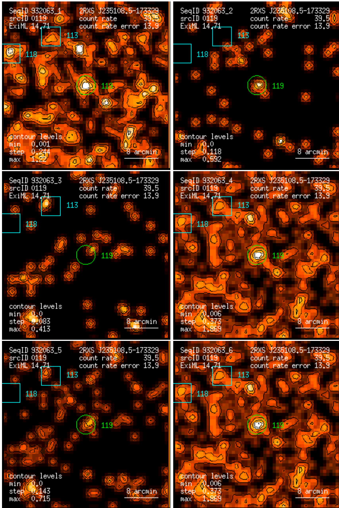
Figure 119: RASS 932063: detection 0119: band rate images, Gaussian filter: (1) PSPC channels 11 – 41, (2) 52 – 90, (3) 91 – 201, (4) 11 – 235, (5) 52 – 201, (6) 11 – 201. Broad band rates in counts/ks. Band rate contour levels in counts/ks/arcmin 2 .
