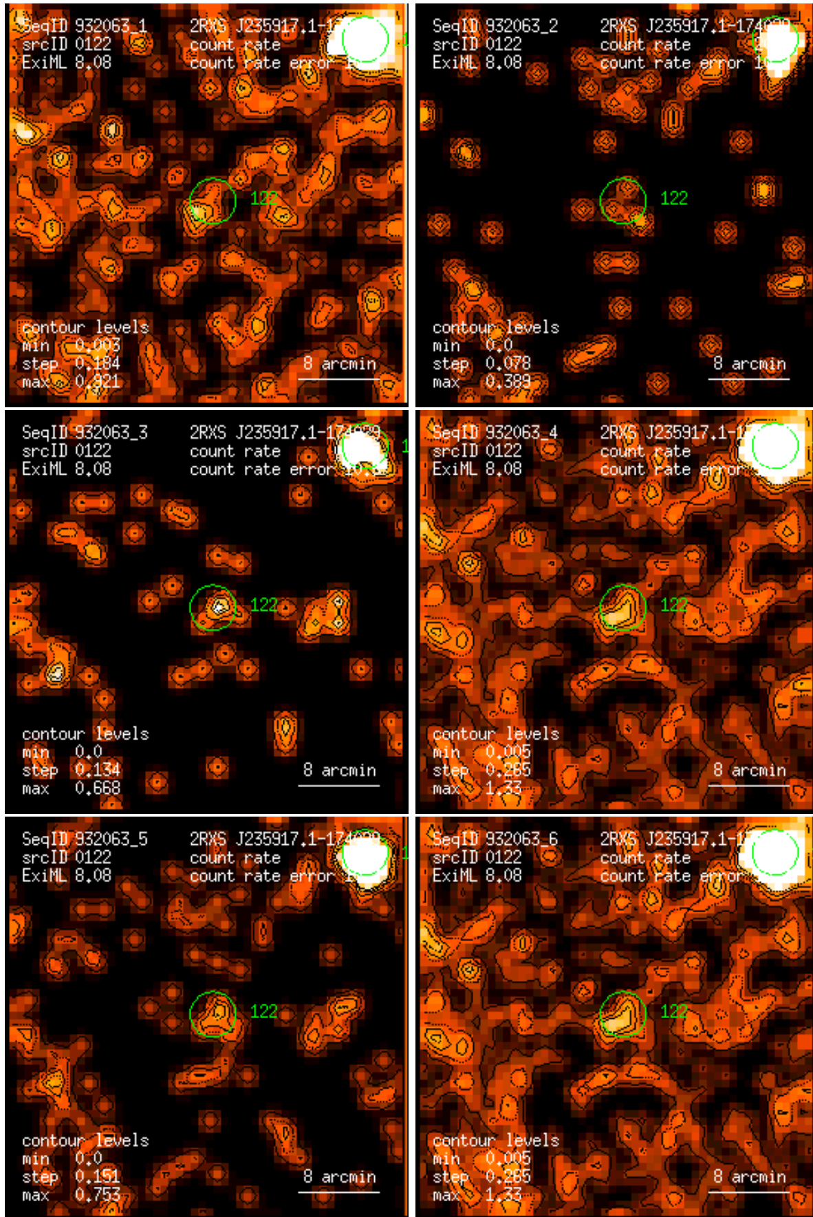
Figure 122: RASS 932063: detection 0122: band rate images, Gaussian filter: (1) PSPC channels 11 – 41, (2) 52 – 90, (3) 91 – 201, (4) 11 – 235, (5) 52 – 201, (6) 11 – 201. Broad band rates in counts/ks. Band rate contour levels in counts/ks/arcmin 2 .
