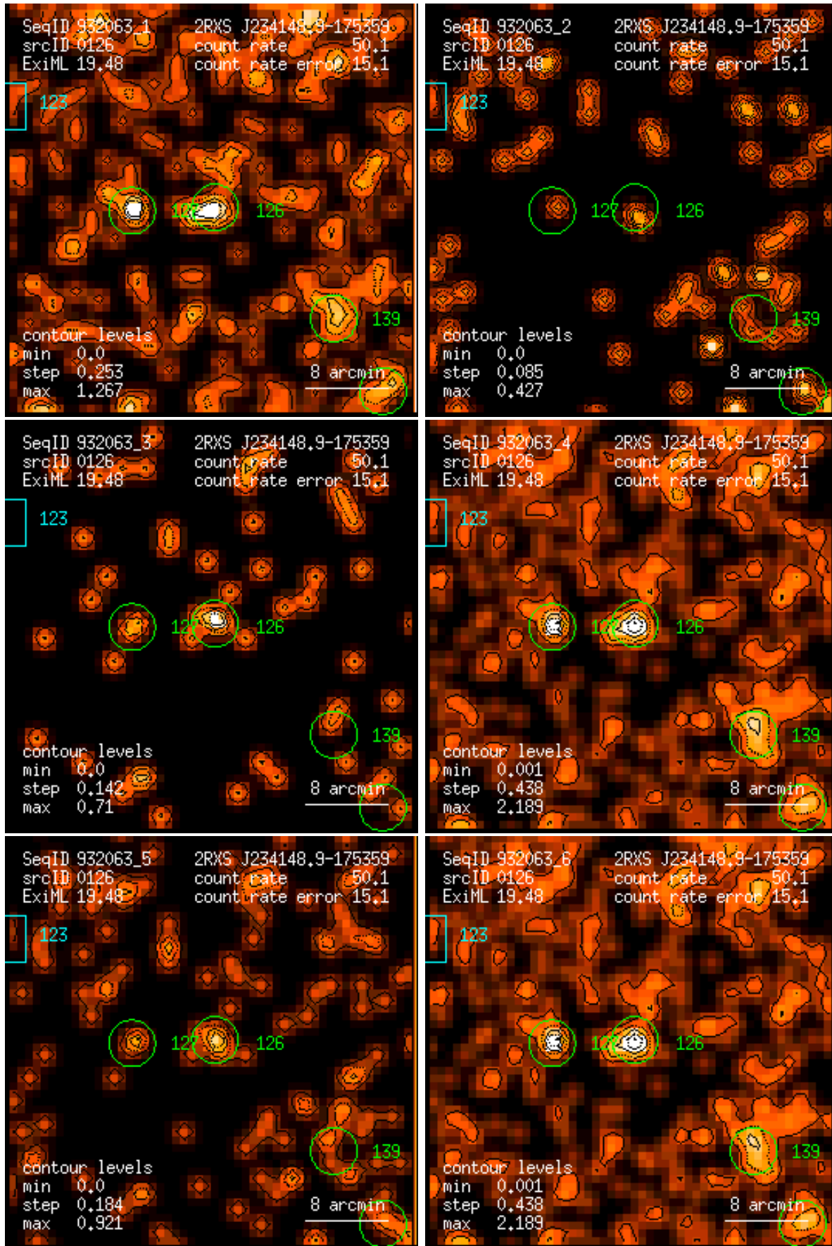
Figure 126: RASS 932063: detection 0126: band rate images, Gaussian filter: (1) PSPC channels 11 – 41, (2) 52 – 90, (3) 91 – 201, (4) 11 – 235, (5) 52 – 201, (6) 11 – 201. Broad band rates in counts/ks. Band rate contour levels in counts/ks/arcmin 2 .
