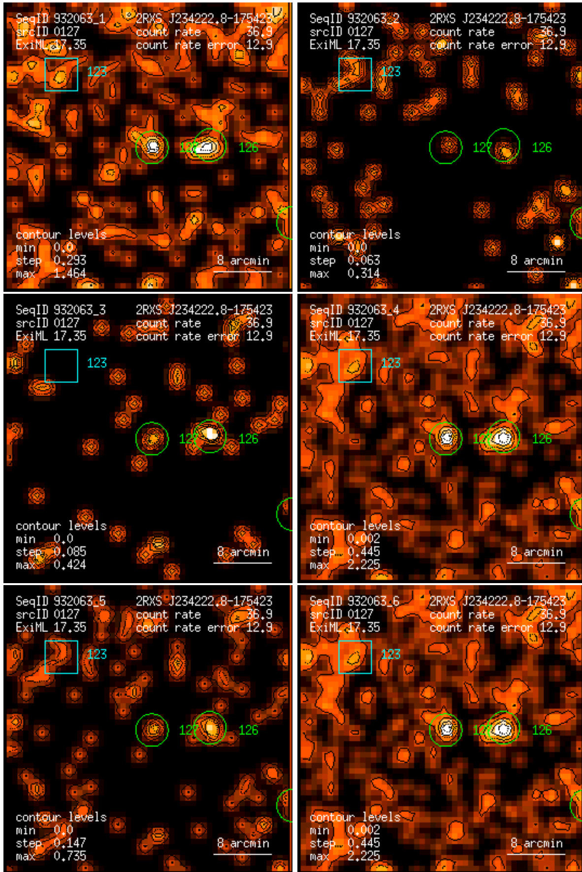
Figure 127: RASS 932063: detection 0127: band rate images, Gaussian filter: (1) PSPC channels 11 – 41, (2) 52 – 90, (3) 91 – 201, (4) 11 – 235, (5) 52 – 201, (6) 11 – 201. Broad band rates in counts/ks. Band rate contour levels in counts/ks/arcmin 2 .
